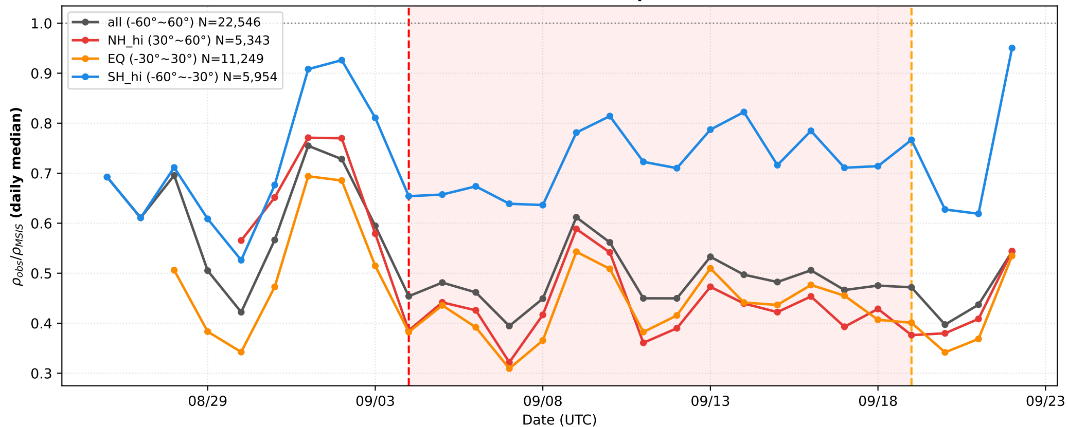
2019 SH SSW Swarm-B — Lat-band Comparison LT=1.0h ±1.0h
