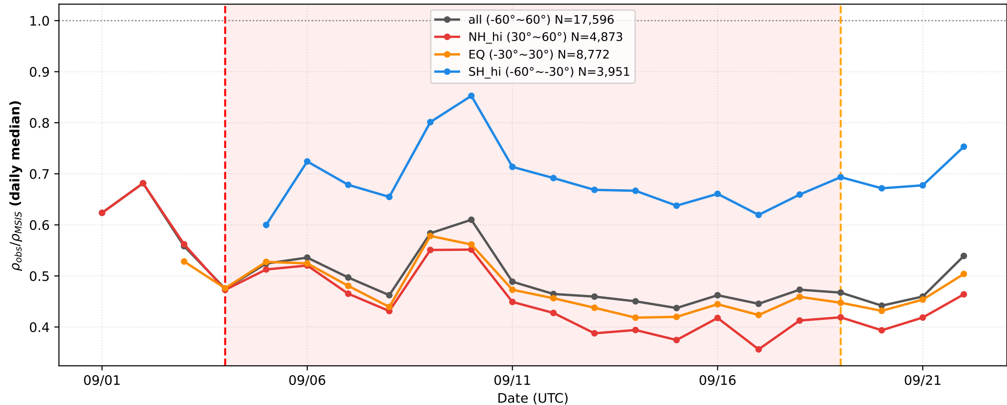
2019 SH SSW Swarm-B — Lat-band Comparison LT=12.5h \pm 1.0h
