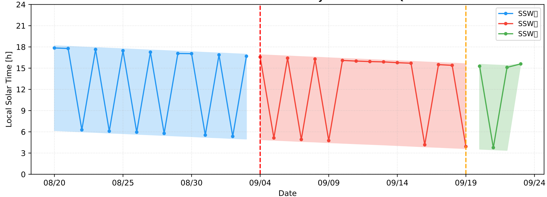
2019 SH SSW Swarm-C — Daily Median LT \pm IQR
