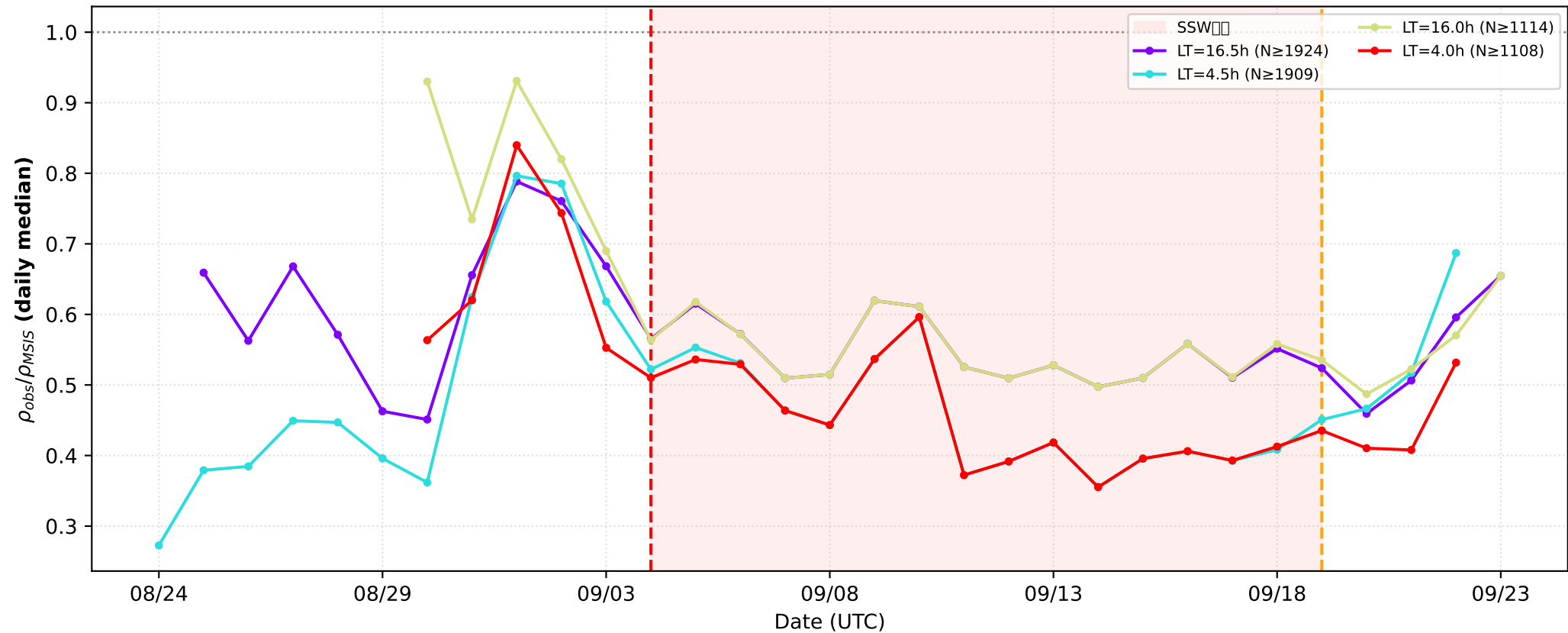
2019 SH SSW Swarm-C — Multi-LT Overlay \pm 1.0h bins
