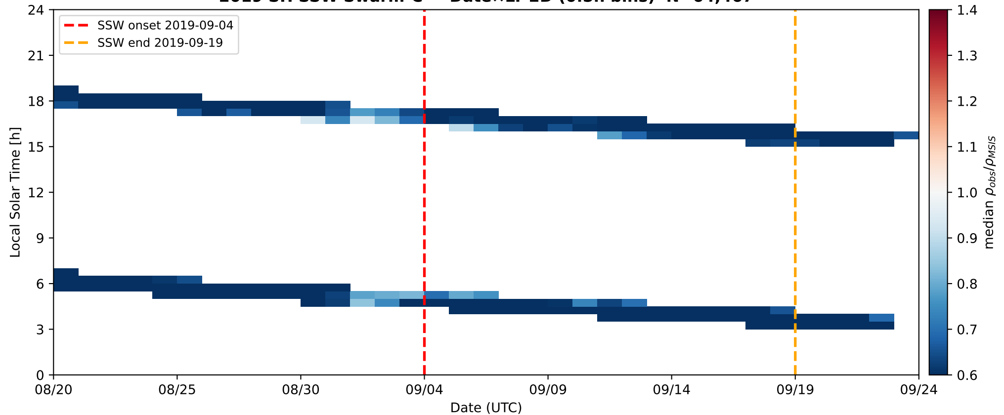
2019 SH SSW Swarm-C — Date×LT 2D (0.5h bins) N=64,467
