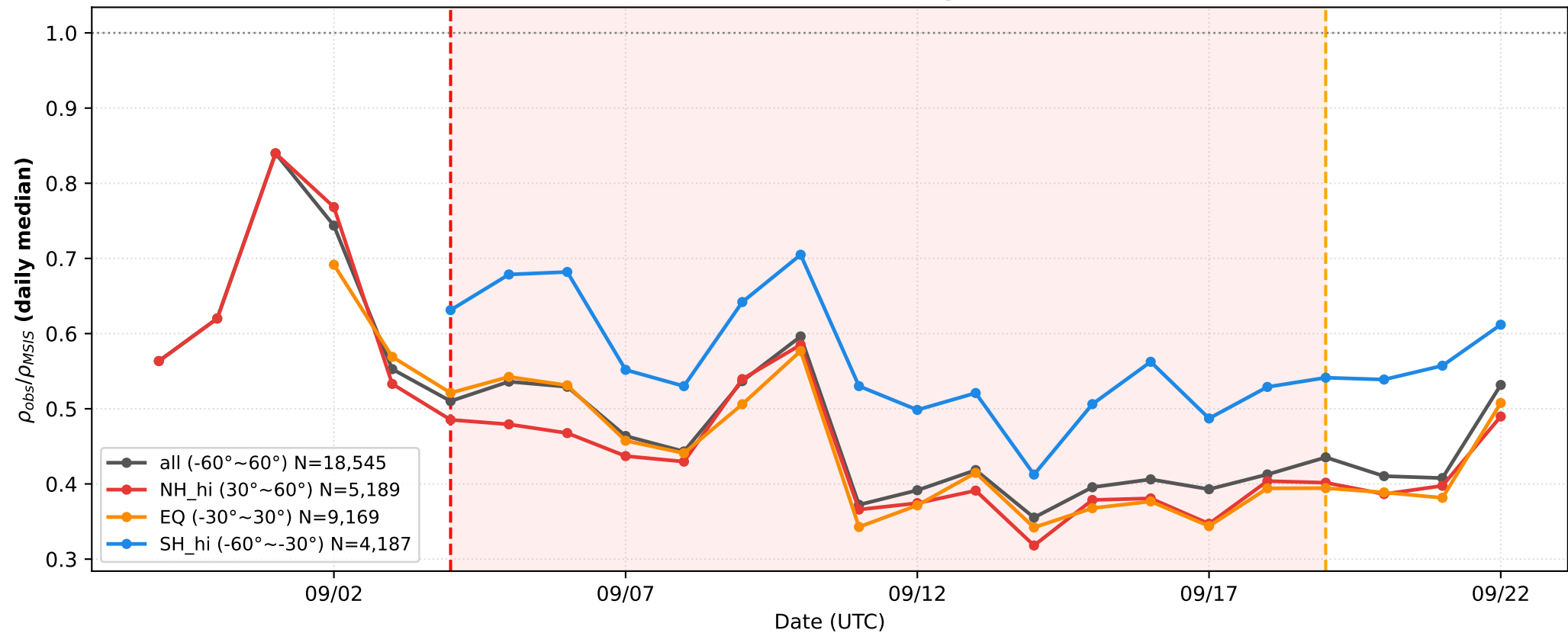
2019 SH SSW Swarm-C — Lat-band Comparison LT=4.0h \pm 1.0h
