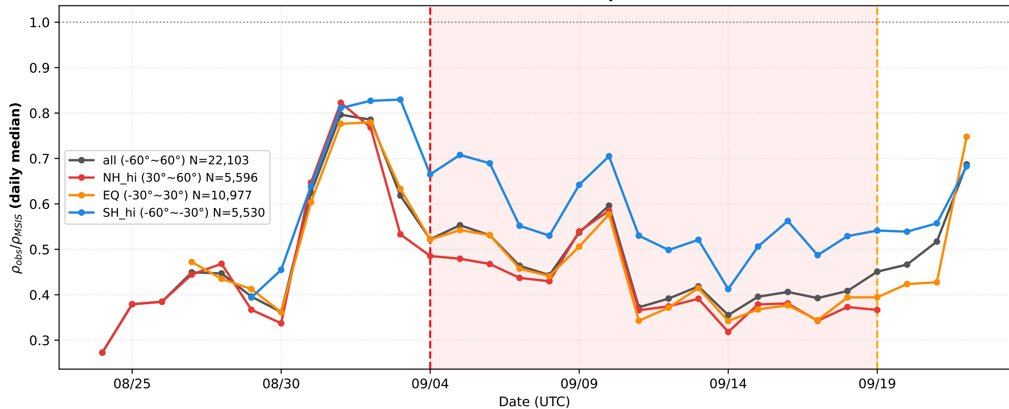
2019 SH SSW Swarm-C — Lat-band Comparison LT=4.5h \pm 1.0h
