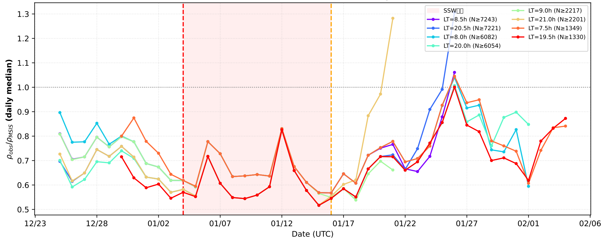
2021 NH SSW Swarm-C — Multi-LT Overlay \pm 1.5h bins
