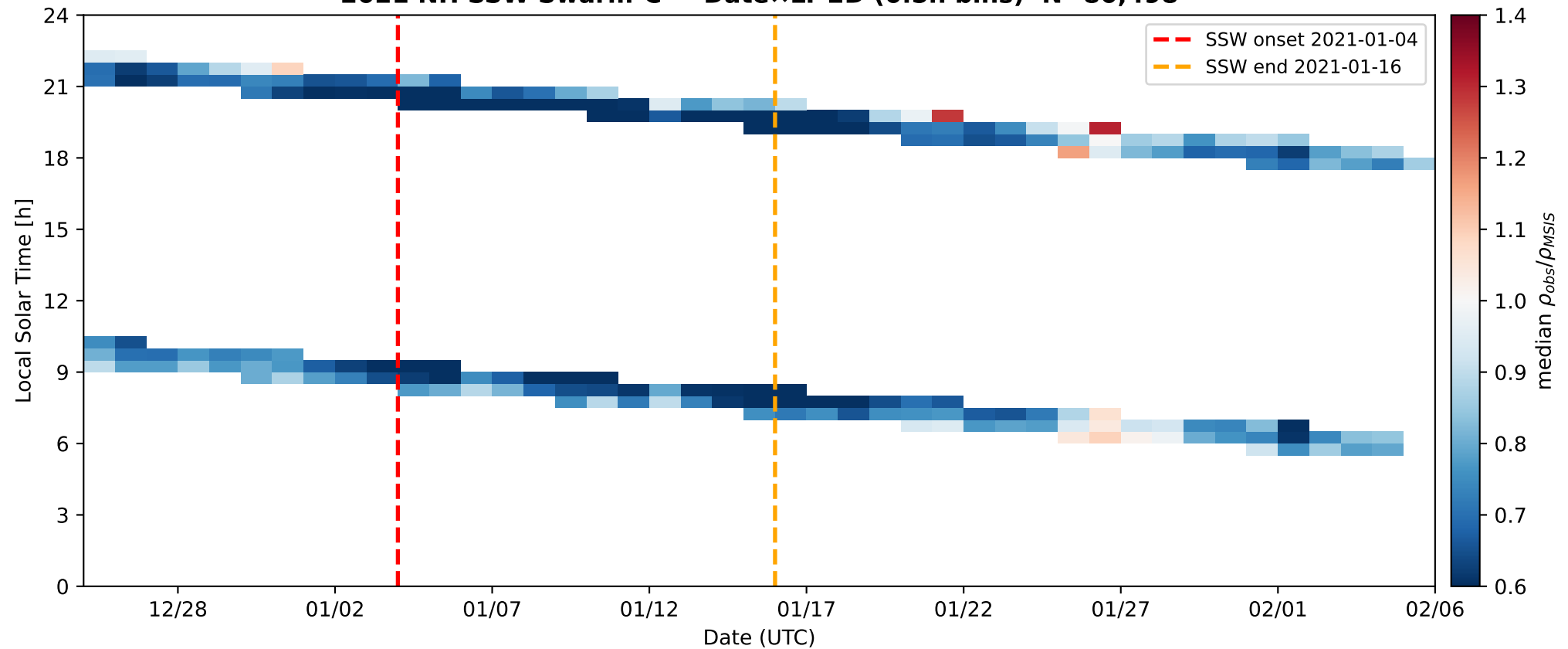
2021 NH SSW Swarm-C — Date×LT 2D (0.5h bins) N=80,498
