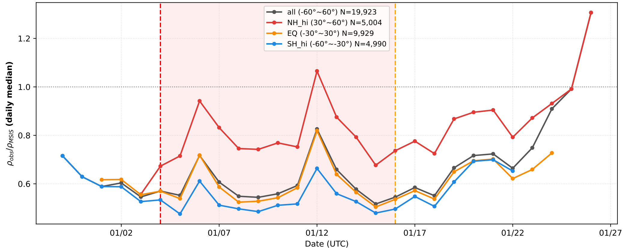
2021 NH SSW Swarm-C — Lat-band Comparison LT=20.0h \pm 1.0 h
