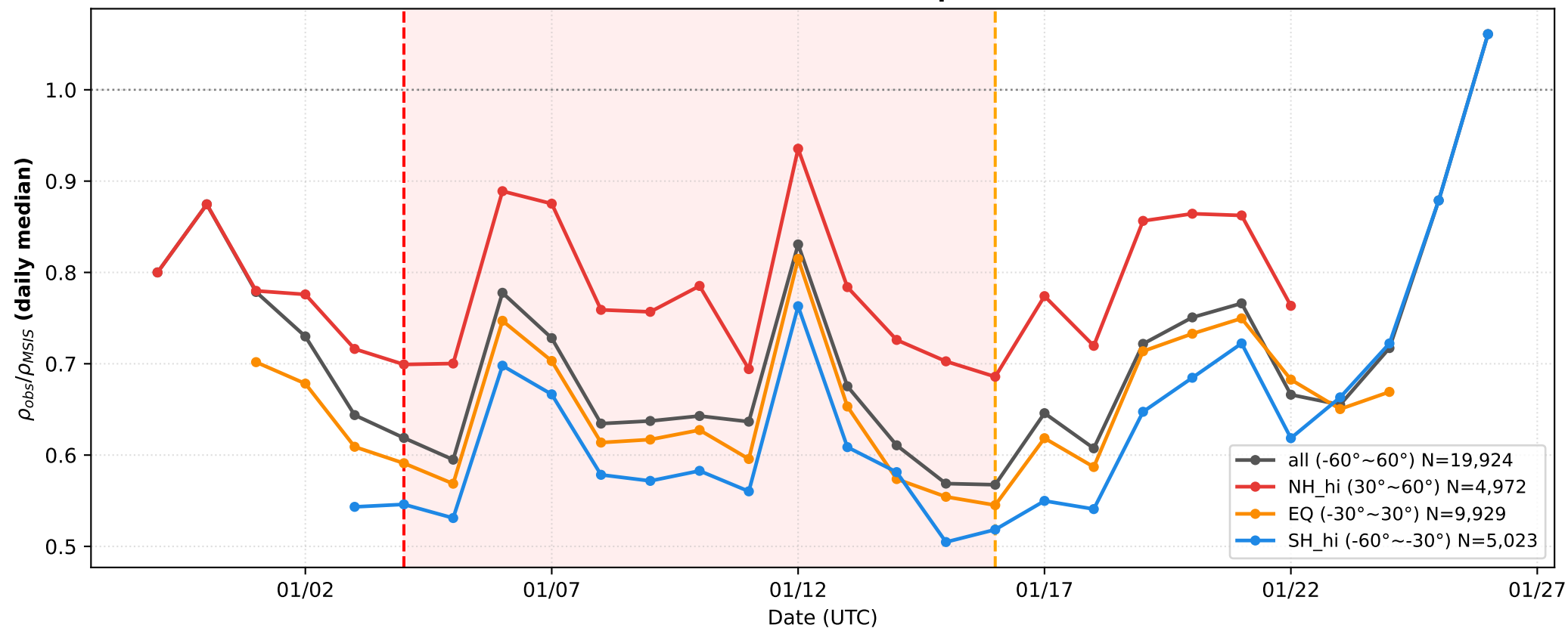
2021 NH SSW Swarm-C — Lat-band Comparison LT=8.0h ±1.0h
