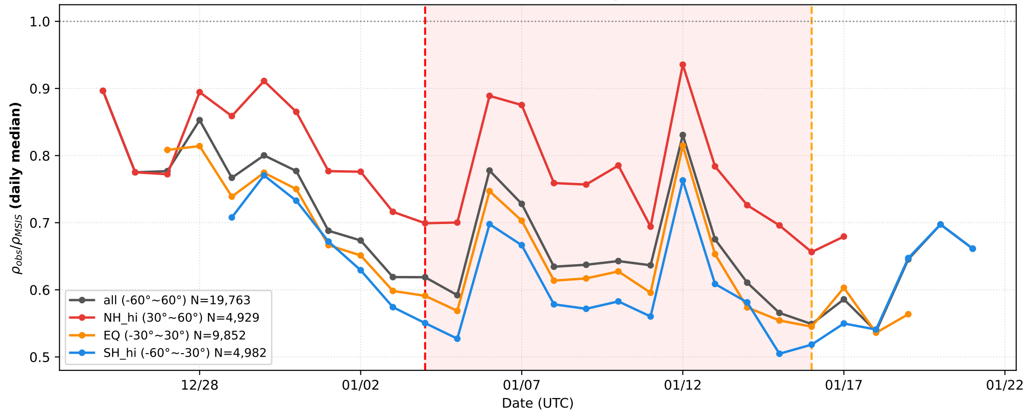
2021 NH SSW Swarm-C — Lat-band Comparison LT=8.5h \pm 1.0h
