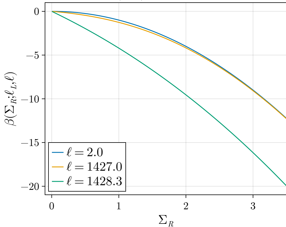
(a-1) \beta -function
