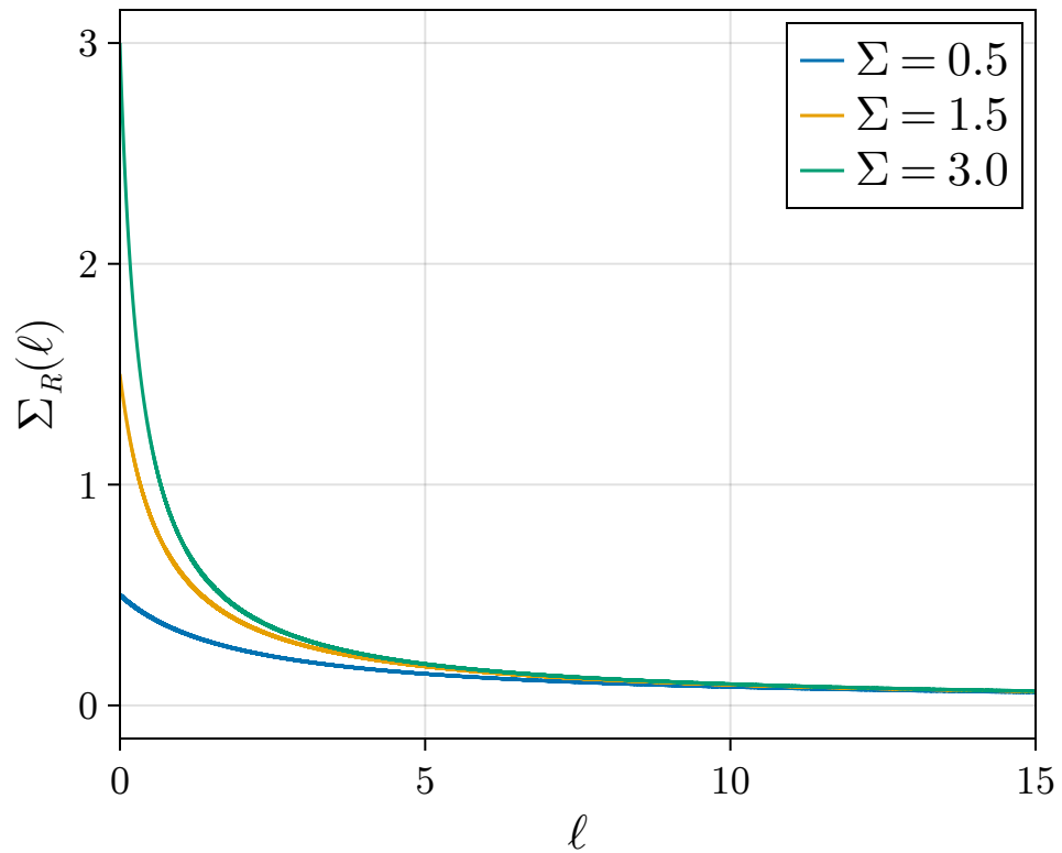
(a-2) RG flow of \Sigma_R
