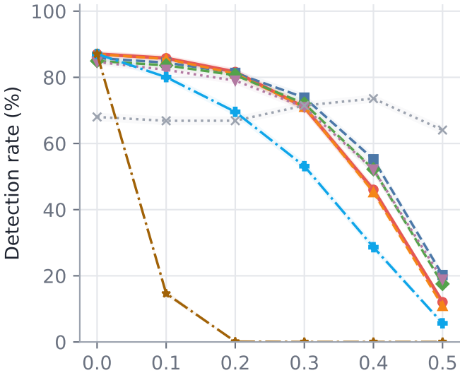
Detection of gradual fatigue drift
