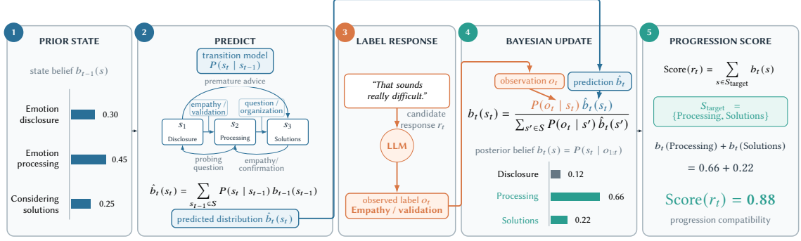
Fig. 2. Schematic example of candidate-response evaluation in the Dialogue Progression Scoring Module. The state distribution through the previous turn is predicted using the transition model and then updated with the observation label derived from the candidate response. The blue path indicates where the predicted distribution enters the update equation, and the orange path indicates where the observation label enters it. In this example, the probabilities of the target states Processing and Solutions in the updated distribution are summed to obtain Score = 0.88.
