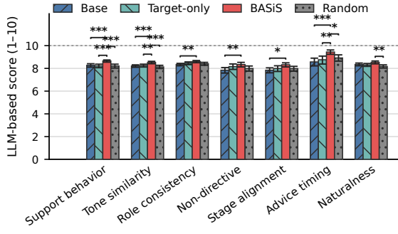
Fig. 6. LLM-based evaluation results for ESConv-DailyDialog. Bars show condition means and bootstrap 95% confidence intervals. Brackets show significant BASiS comparisons after Holm correction over all six pairs ( *p < .05 , **p < .01 , ***p < .001 ).
