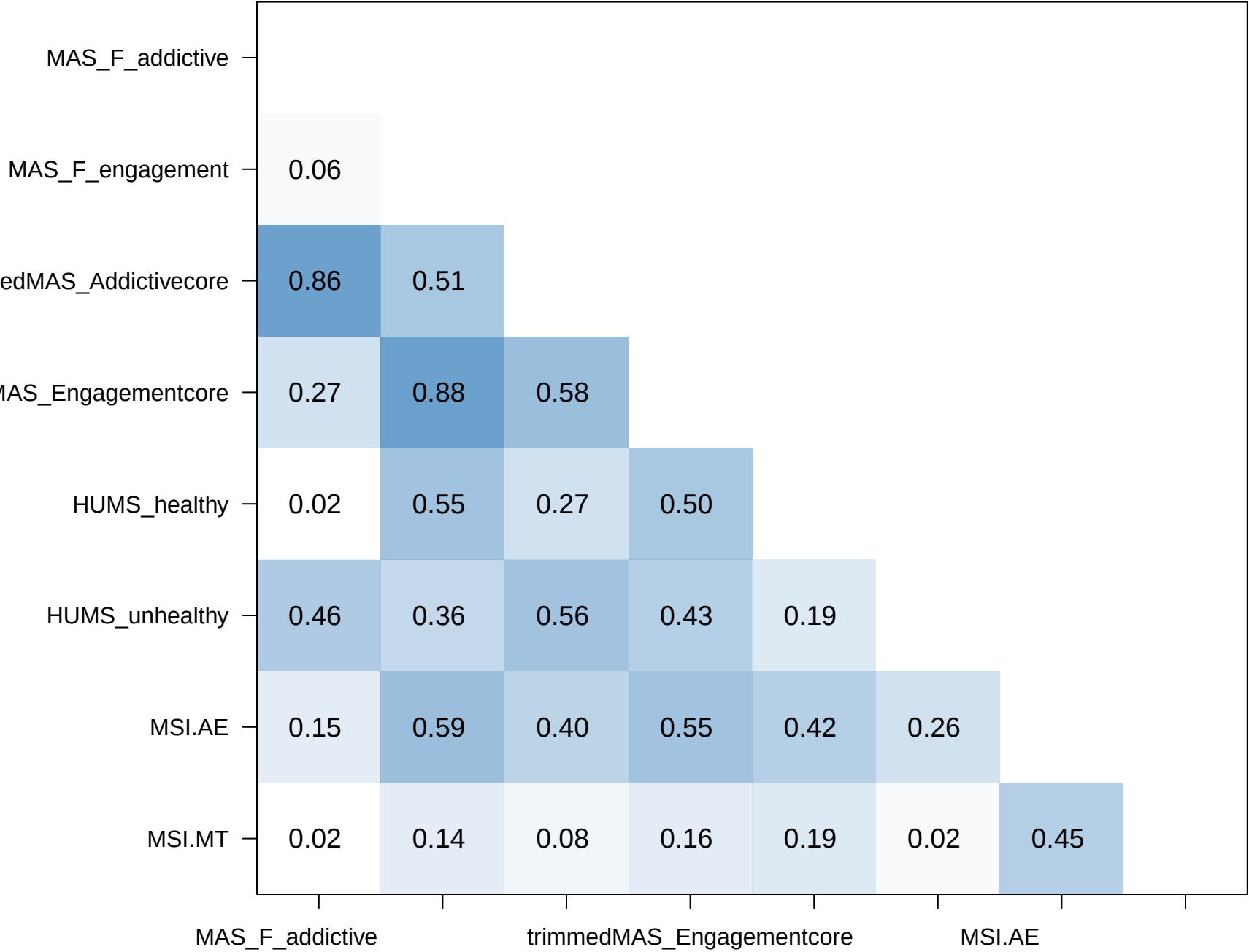
Correlation plot
