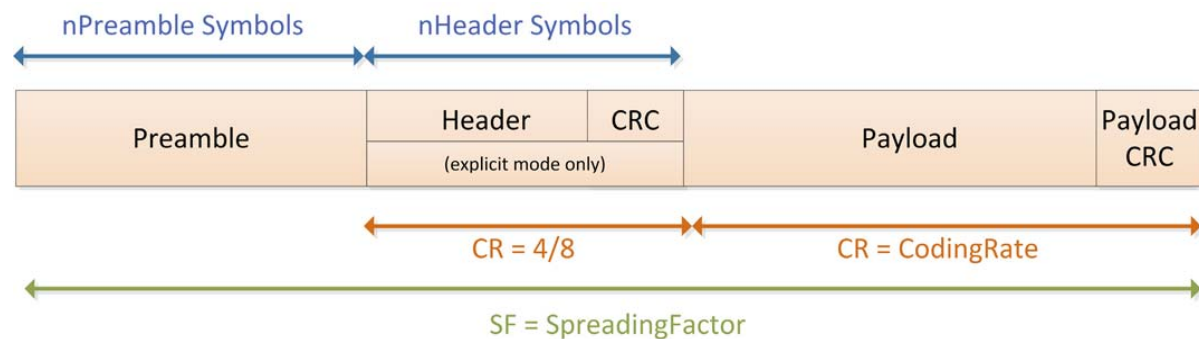
Figure 5. LoRa™ Packet Structure
