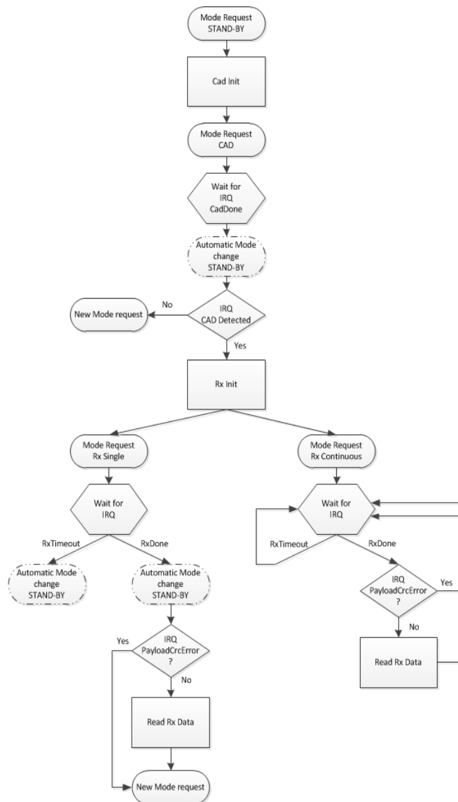
Figure 10. LoRa™ CAD flow
