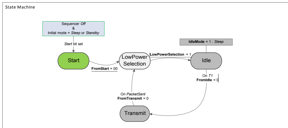
Figure 53. Beacon Mode State Machine
