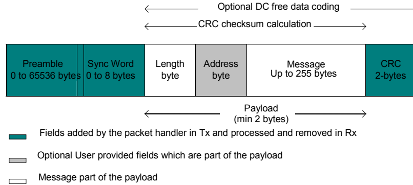
Figure 34. Variable Length Packet Format
