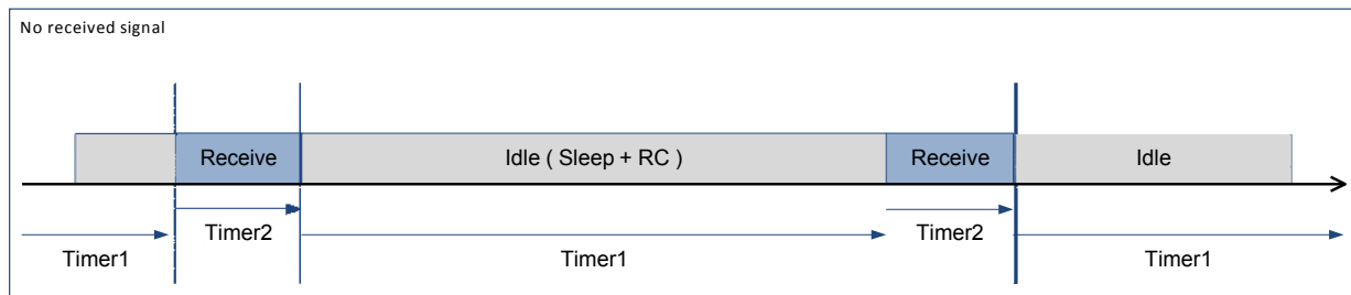
Figure 45. Listen Mode with No Preamble Received
