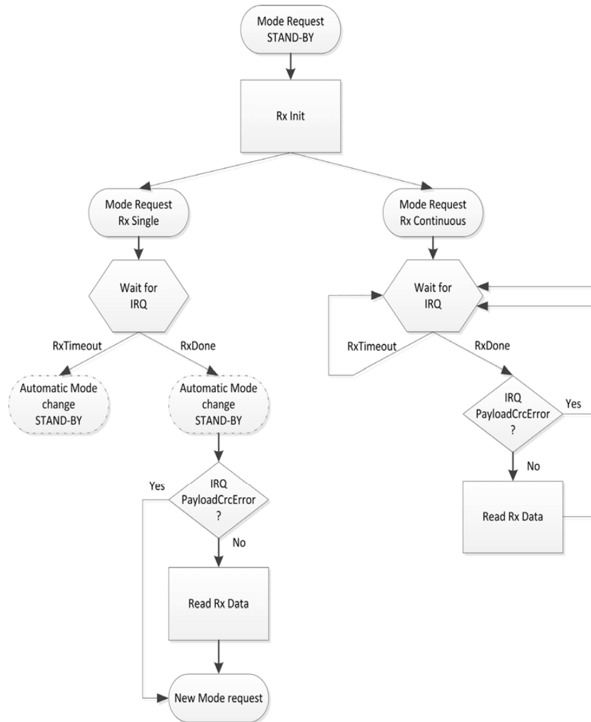
Figure 9. LoRa™ receive sequence.
