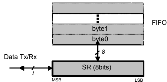
Figure 26. FIFO and Shift Register (SR)
