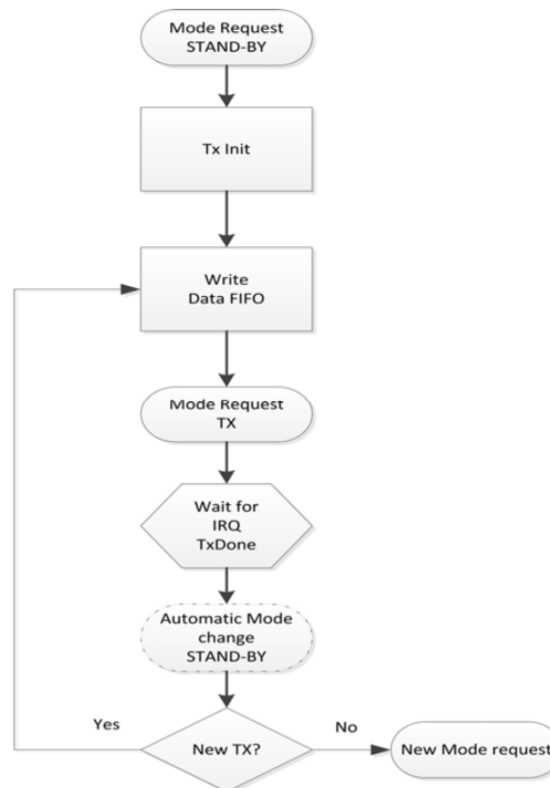
Figure 8. LoRa™ modulation transmission sequence.
