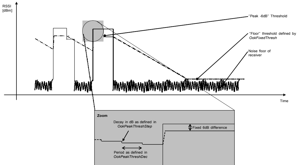
Figure 13. OOK Peak Demodulator Description
