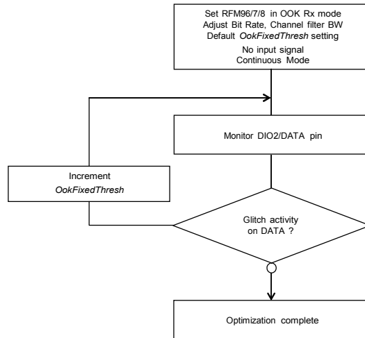
Figure 14. Floor Threshold Optimization
