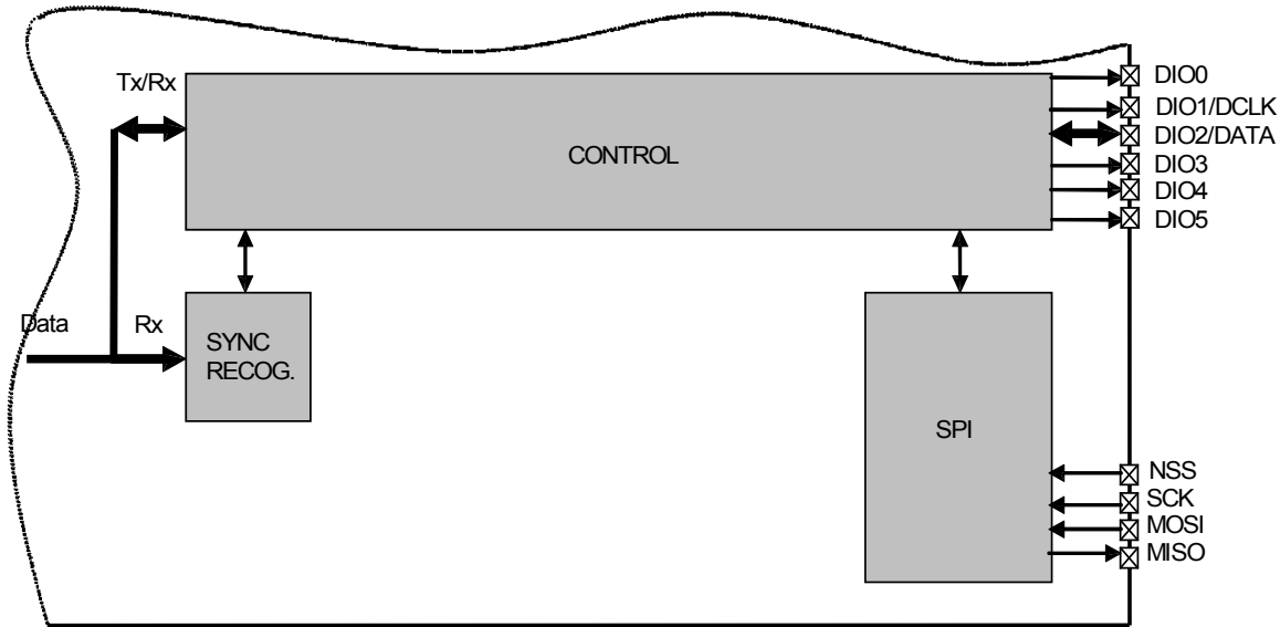
Figure 29. Continuous Mode Conceptual View
