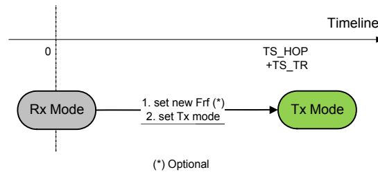
Figure 20. Rx to Tx Turnaround
