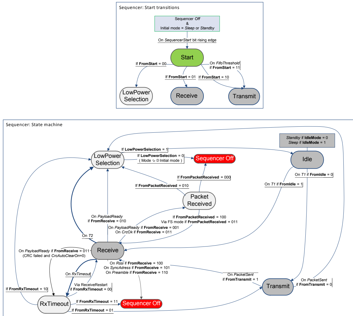
Figure 24. Sequencer State Machine
