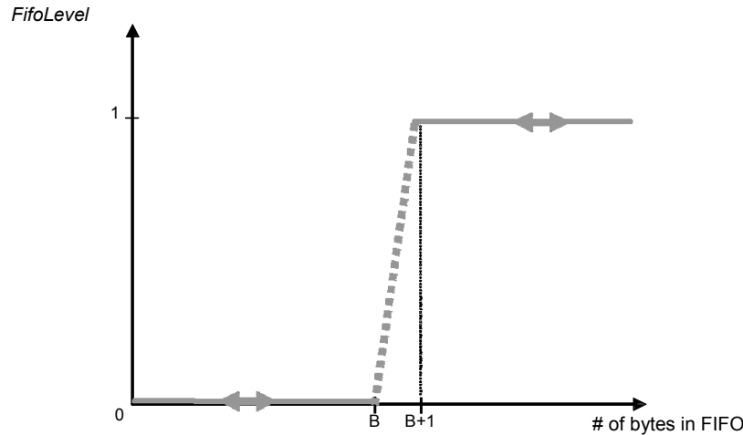
Figure 27. FifoLevel IRQ Source Behavior
