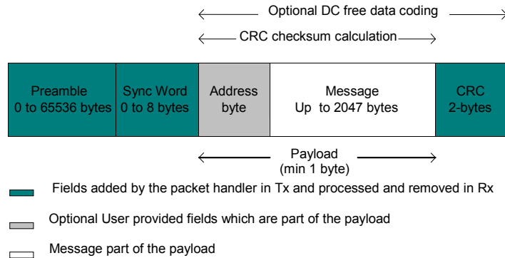
Figure 33. Fixed Length Packet Format
