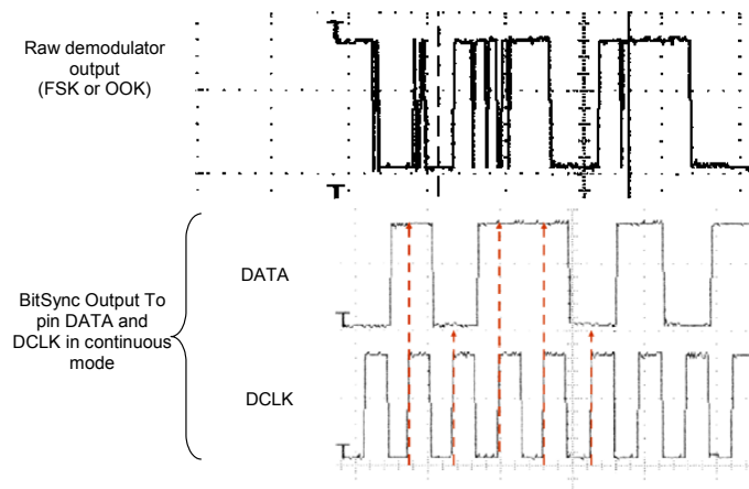
Figure 15. Bit Synchronizer Description
