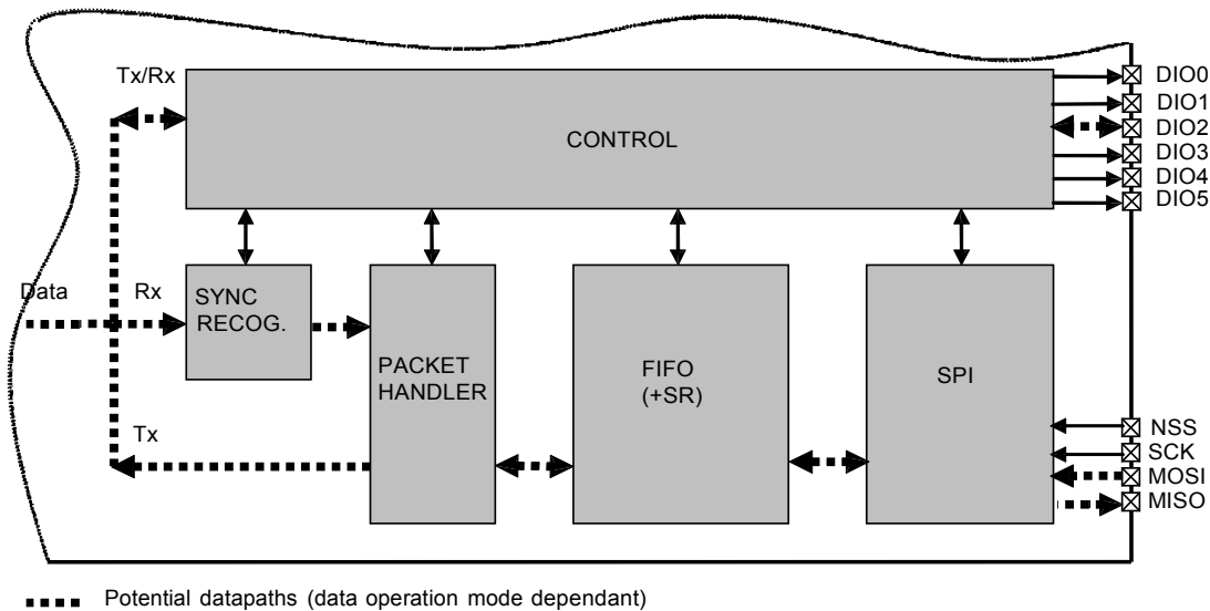
Figure 25. RFM95/96/97/98(W) Data Processing Conceptual View
