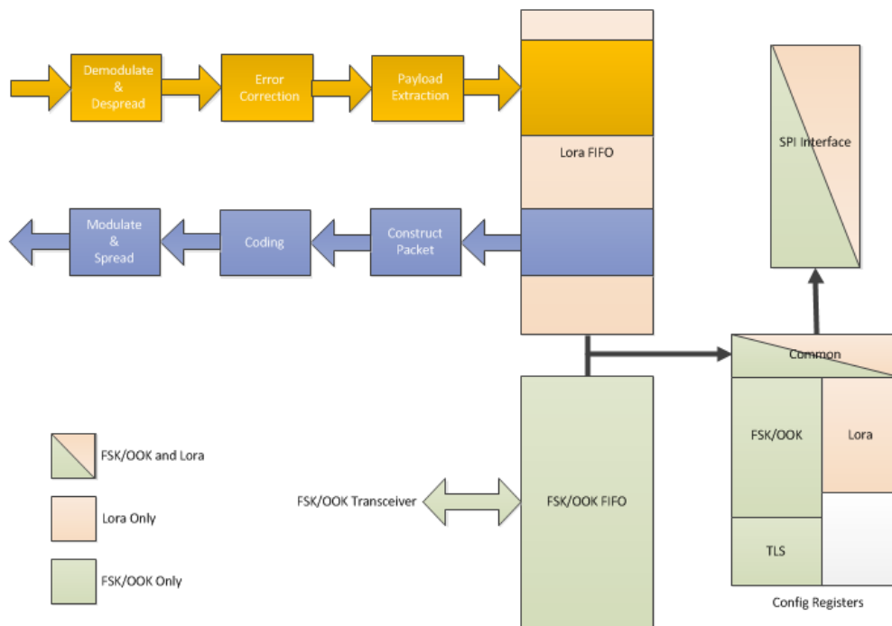
Figure 4. LoRa™ Modem Connectivity
