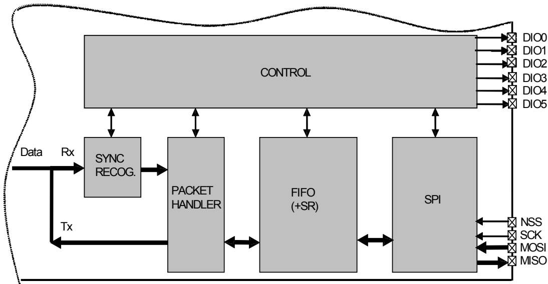
Figure 32. Packet Mode Conceptual View
