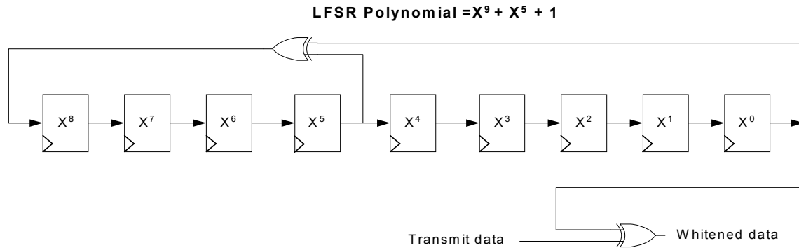
Figure 37. Data Whitening Polynomial
