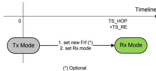
Figure 19. Tx to Rx Turnaround
