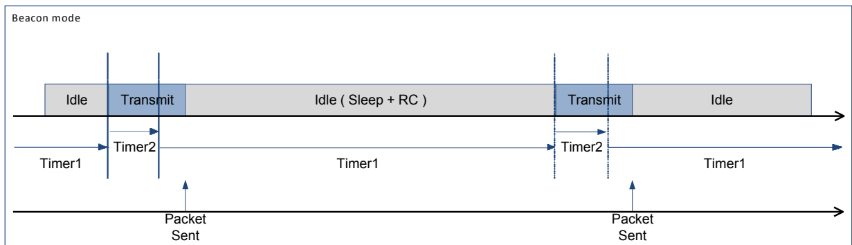
Figure 52. Beacon Mode Timing Diagram
