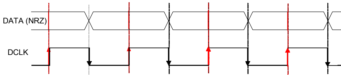
Figure 31. Rx Processing in Continuous Mode
