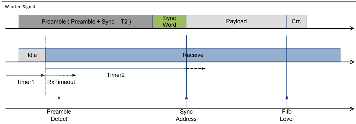
Figure 50. Listen Mode with Preamble Received & Valid SyncAddress
