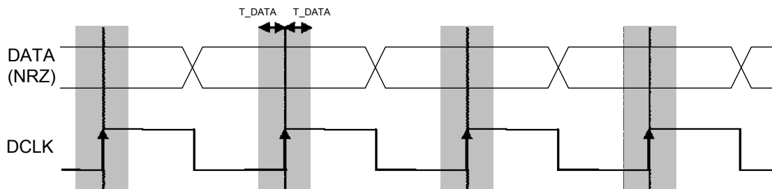
Figure 30. Tx Processing in Continuous Mode
