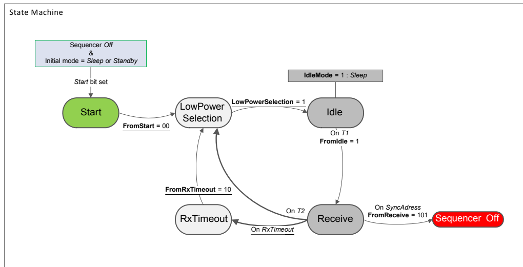
Figure 51. Wake On SyncAddress State Machine
