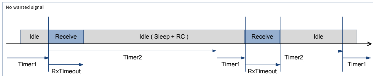
Figure 48. Listen Mode with no SyncAddress Detected
