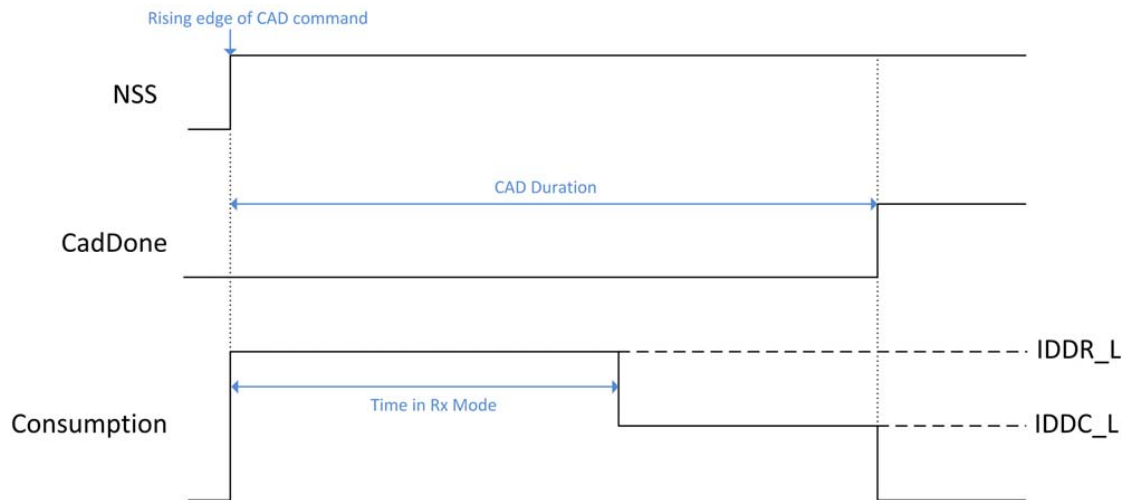
Figure 12. Consumption Profile of the LoRa CAD Process
