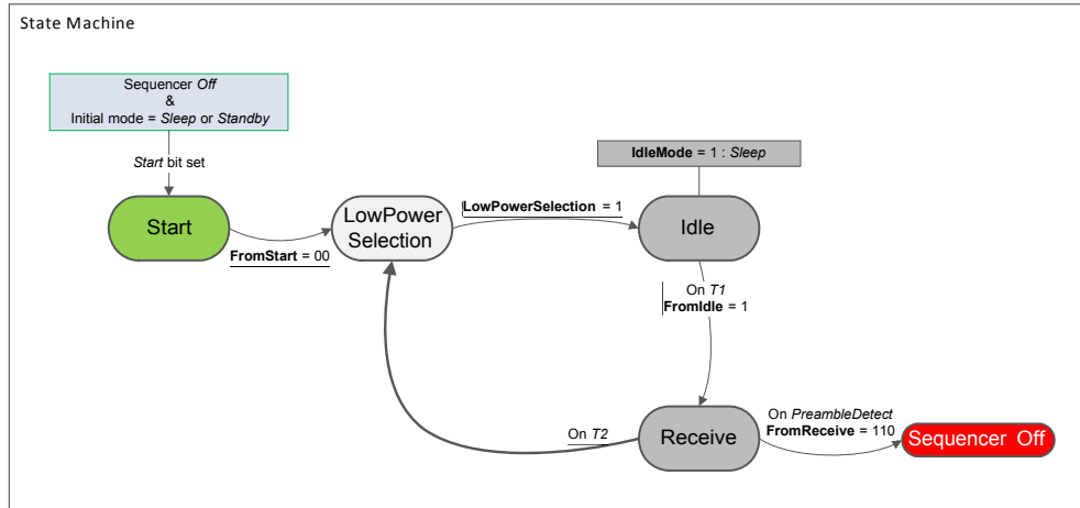
Figure 47. Wake On PreambleDetect State Machine
