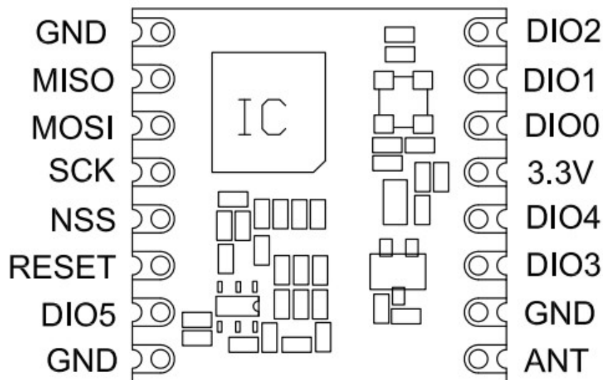
Figure 2. Pin Diagrams
