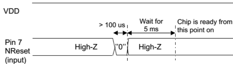
Figure 43. Manual Reset Timing Diagram
