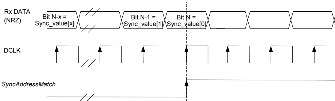
Figure 28. Sync Word Recognition
