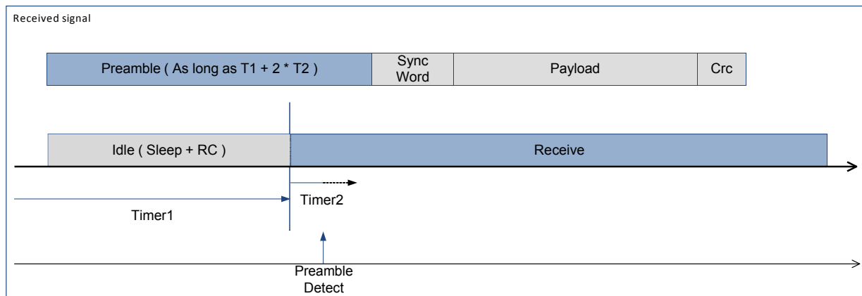
Figure 46. Listen Mode with Preamble Received
