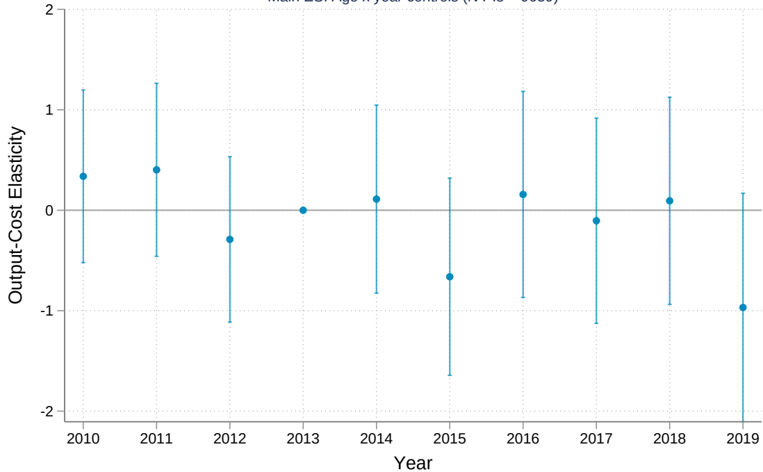
Main ES: Age x year controls (N PIs = 9659)
