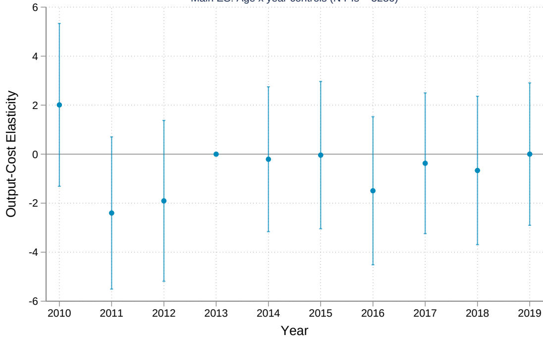
Main ES: Age x year controls (N PIs = 5286)
