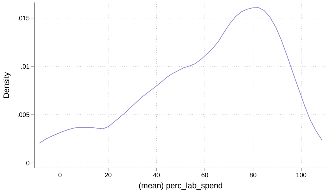
Kernel density estimate
