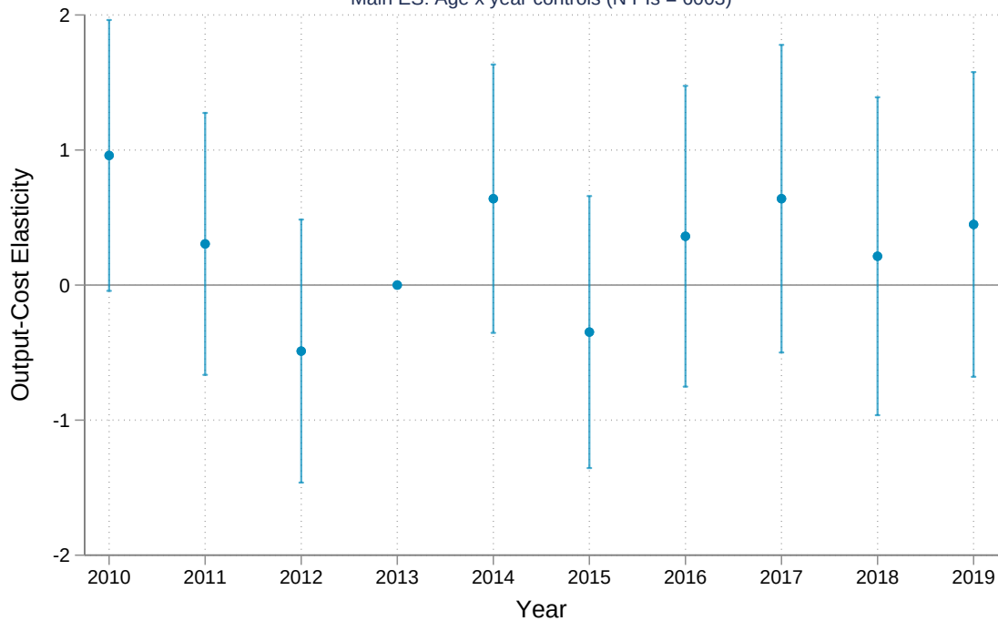
Main ES: Age x year controls (N PIs = 6003)
