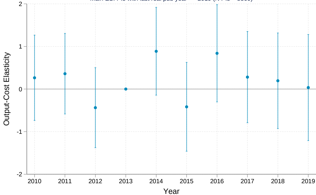
Main ES: Pls with last real pub year \geq 2019 (N Pls = 8869)
