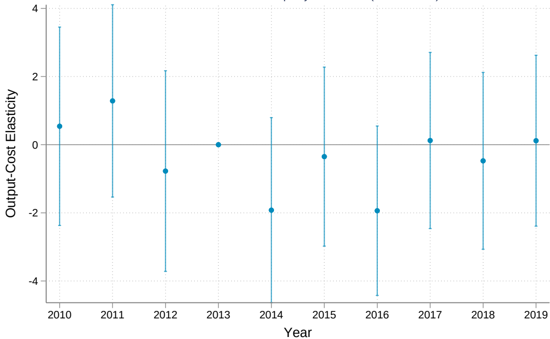
Main ES: Pls with last real pub year \geq 2019 (N Pls = 7401)
