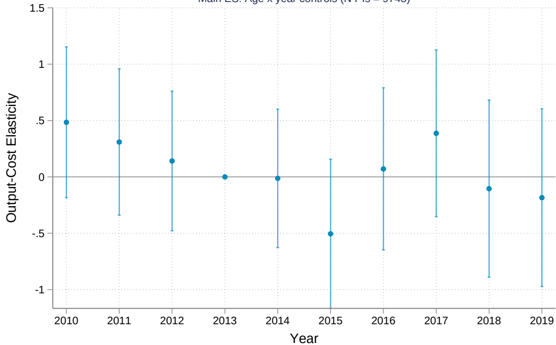
Main ES: Age x year controls (N PIs = 9743)
