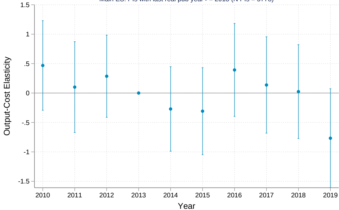
Main ES: PIs with last real pub year \geq 2018 (N PIs = 5778)
