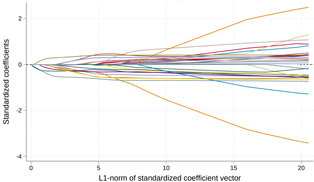
Coefficient paths
