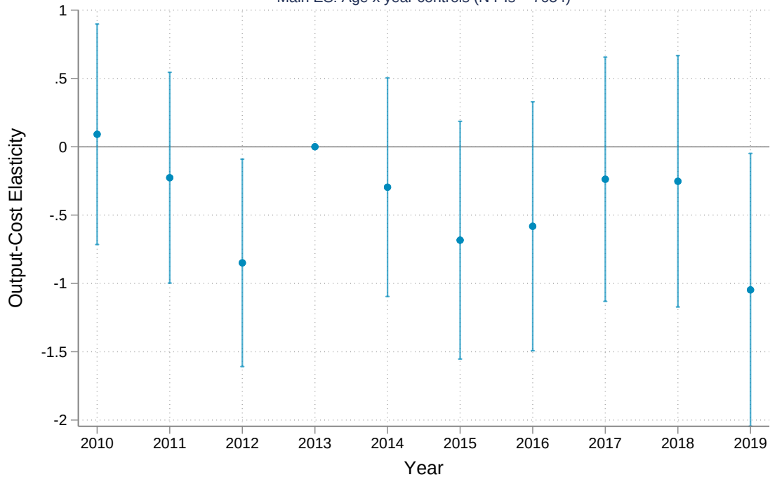
Main ES: Age x year controls (N PIs = 7654)
