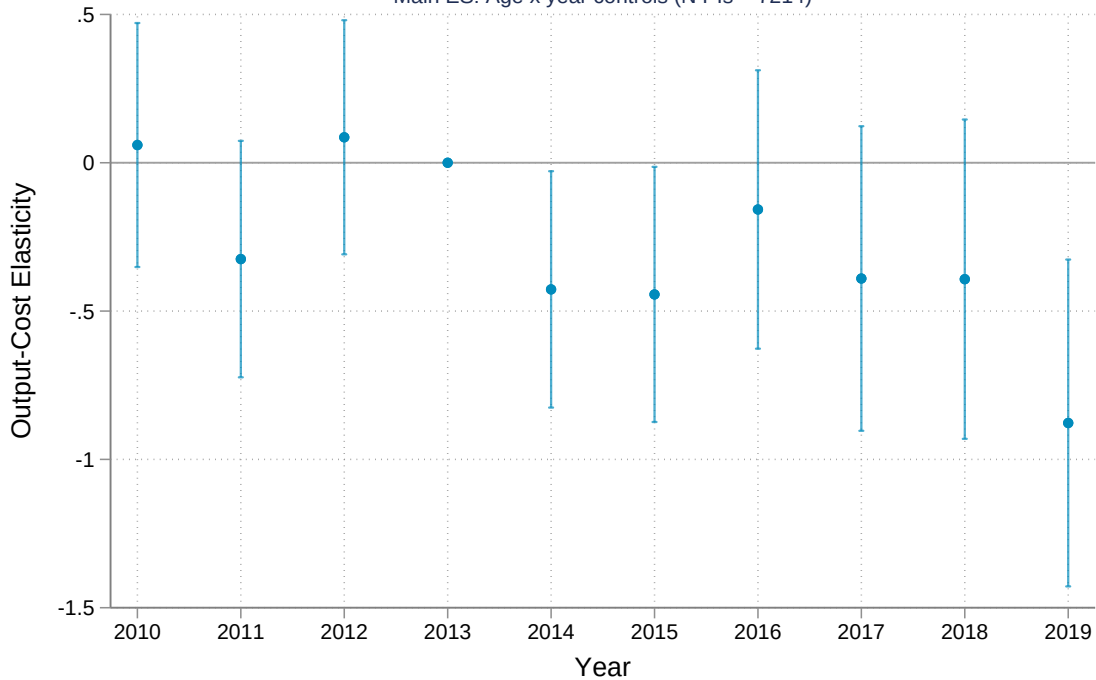
Main ES: Age x year controls (N PIs = 7214)
