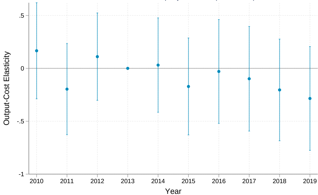
Main ES: PIs with last real pub year \geq 2018 (N PIs = 9263)
