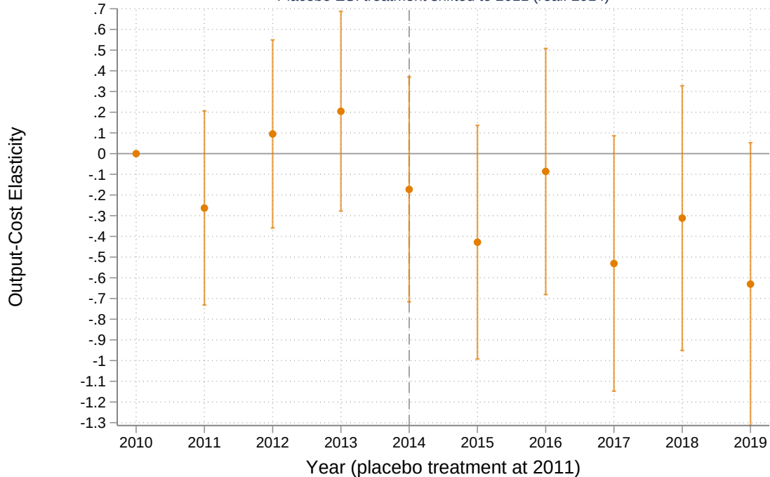
Placebo ES: treatment shifted to 2011 (real: 2014)
