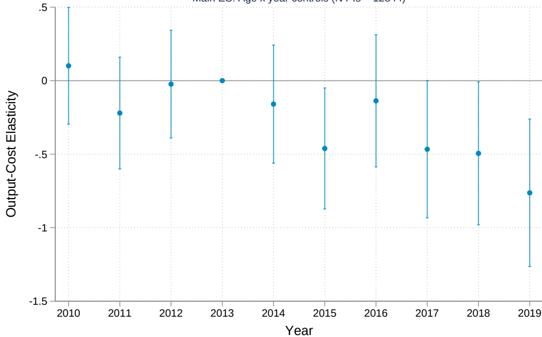
Main ES: Age x year controls (N Pls = 12844)
