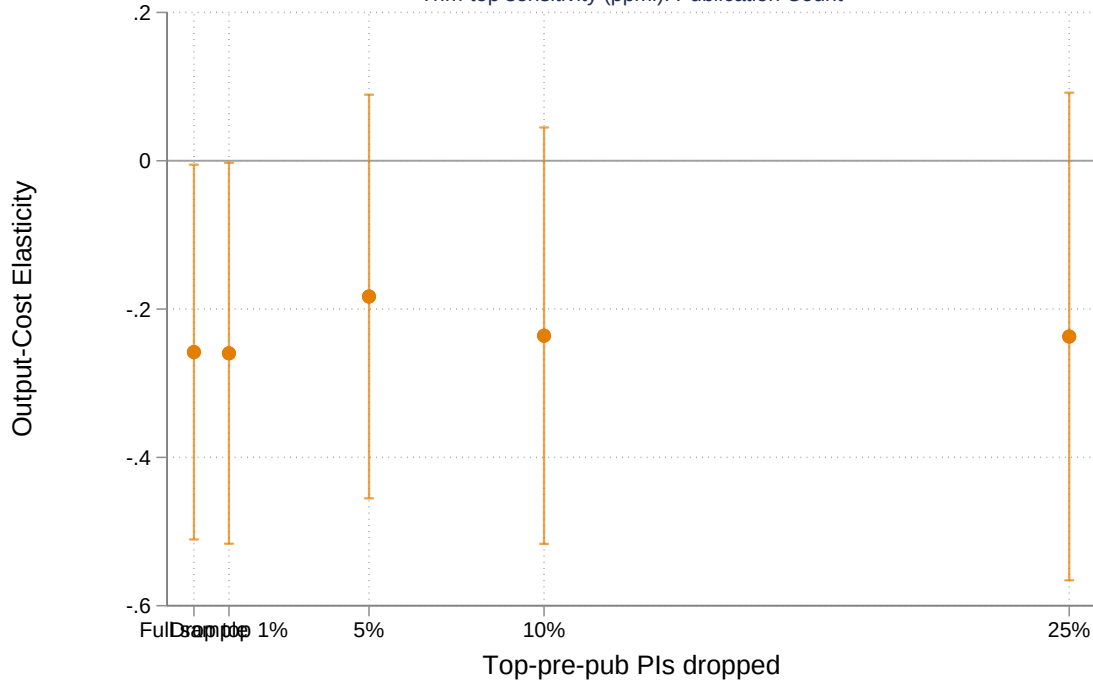
Trim-top sensitivity (ppml): Publication Count
