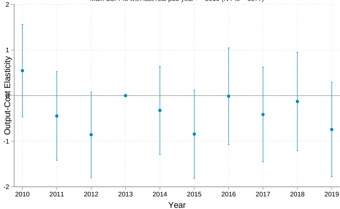
Main ES: PIs with last real pub year \geq 2019 (N PIs = 6577)
