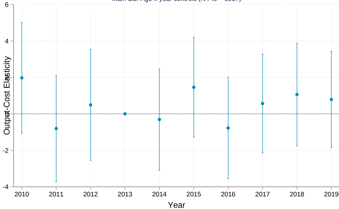
Main ES: Age x year controls (N PIs = 6987)
