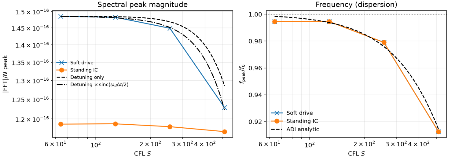
Figure 6.5: Amplitude and frequency of the PEC soft-excitation and standing-wave responses versus CFL number. The amplitude reference curves include the detuning-only model and the combined detuning and discrete-injection model.
