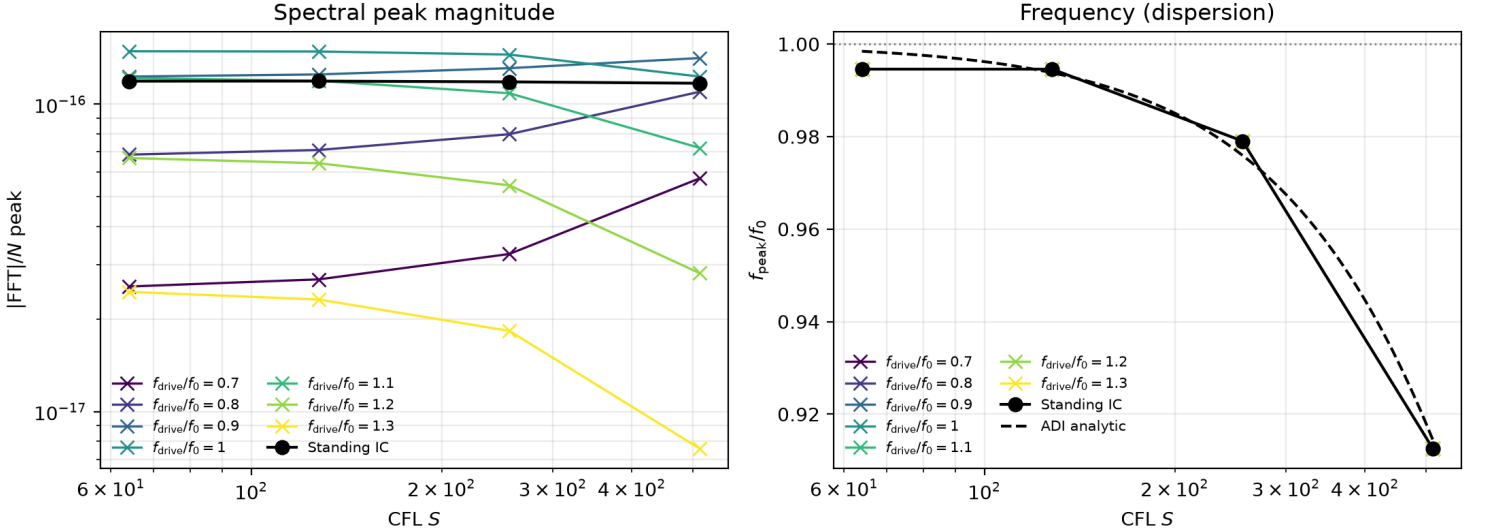
Figure 6.4: Comparison of the frequency of the PEC soft-excitation and PEC standing-wave cases with respect to the CFL number for different excitation frequencies.
