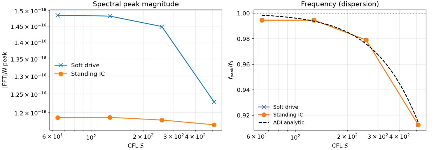
Figure 6.3: Comparison of the amplitude of the PEC soft-excitation and PEC standing-wave cases with respect to the CFL number.
