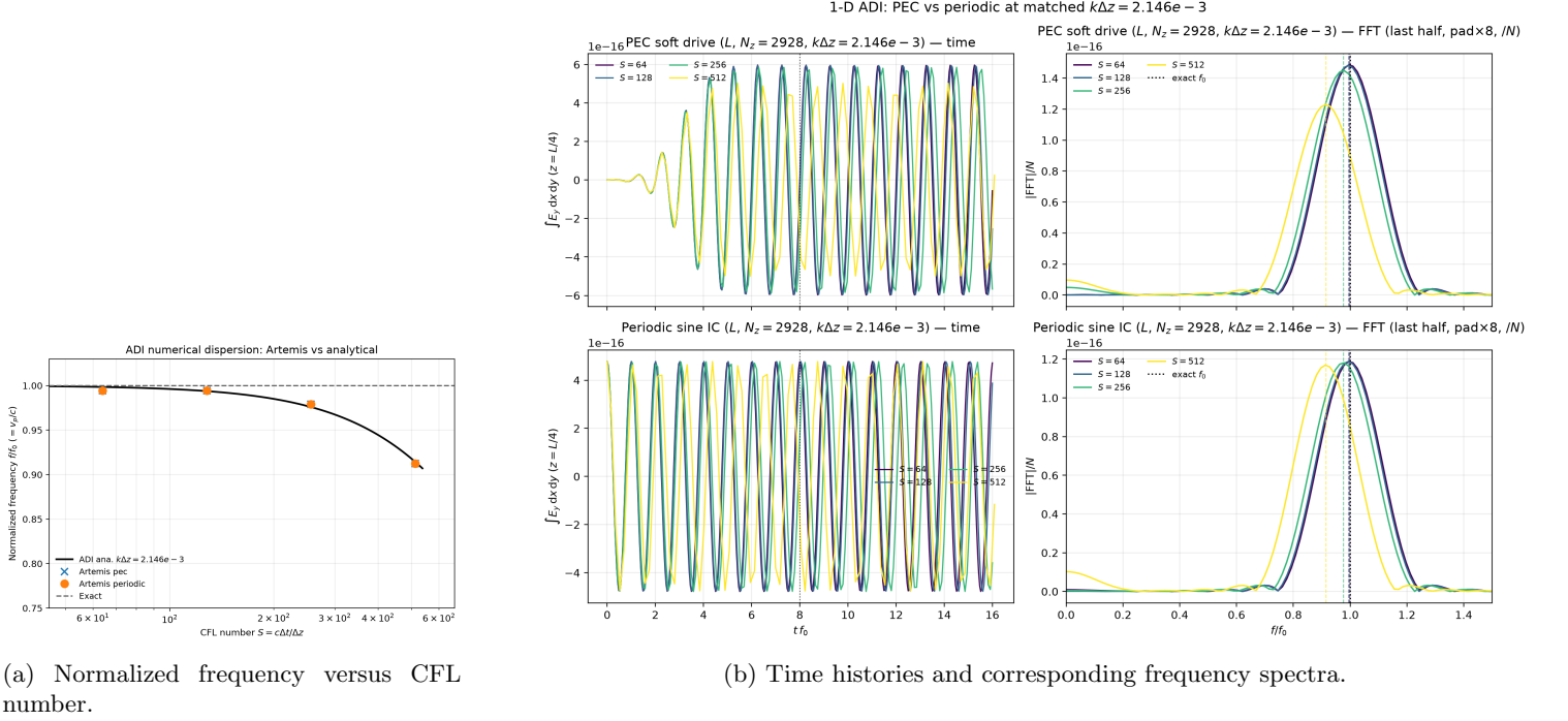
Figure 6.2: Numerical verification of the ADI dispersion relation using PEC soft excitation and periodic traveling waves.
