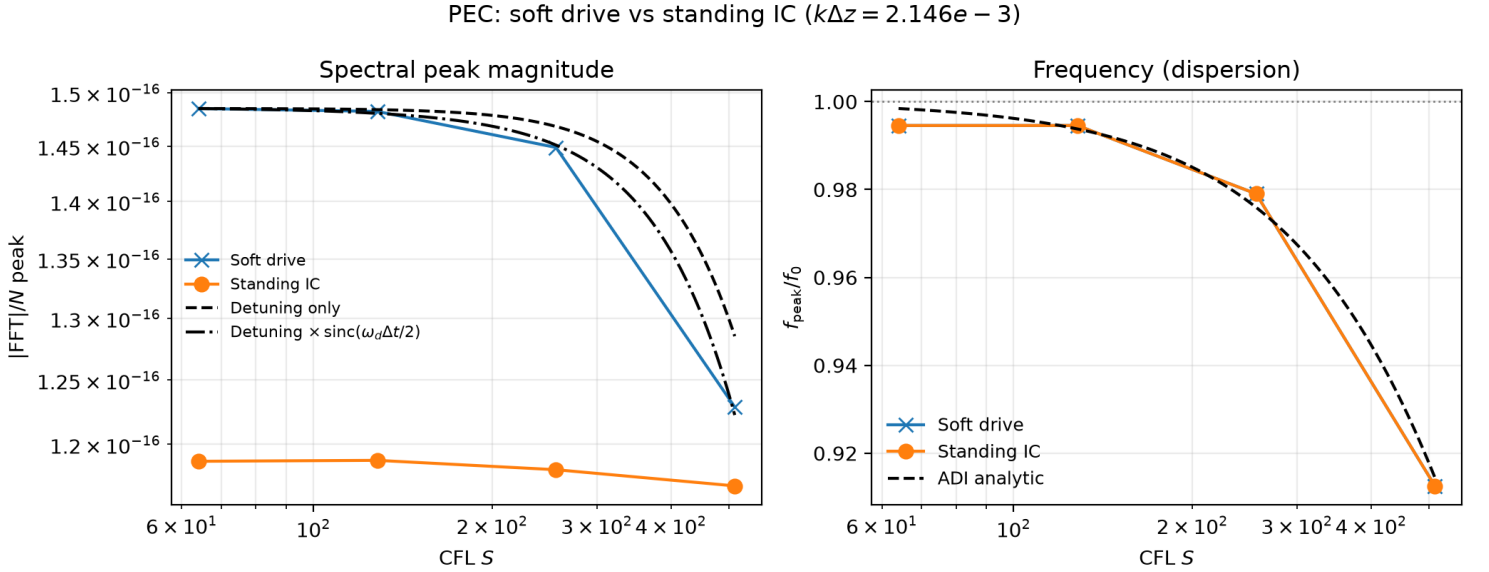
Figure 6.3: Amplitude and frequency of the PEC soft-excitation and standing-wave responses versus CFL number. The amplitude reference curves include the detuning-only model and the combined detuning and discrete-injection model.
