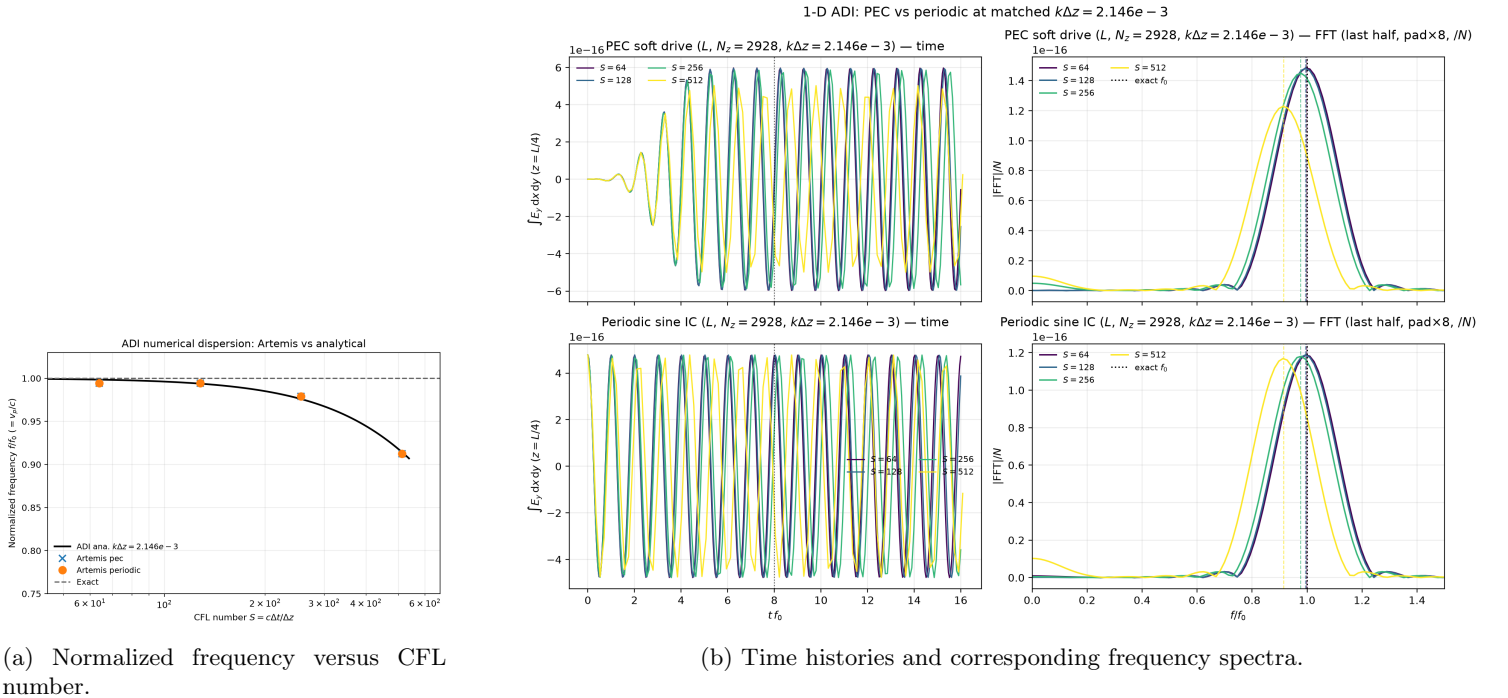
Figure 7.2: Numerical verification of the ADI dispersion relation using PEC soft excitation and periodic traveling waves.
