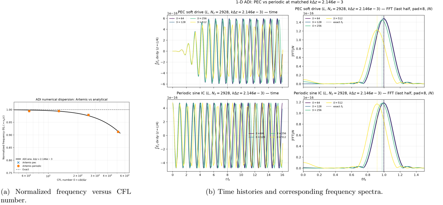
Figure 6.2: Numerical verification of the ADI dispersion relation using PEC soft excitation and periodic traveling waves.
