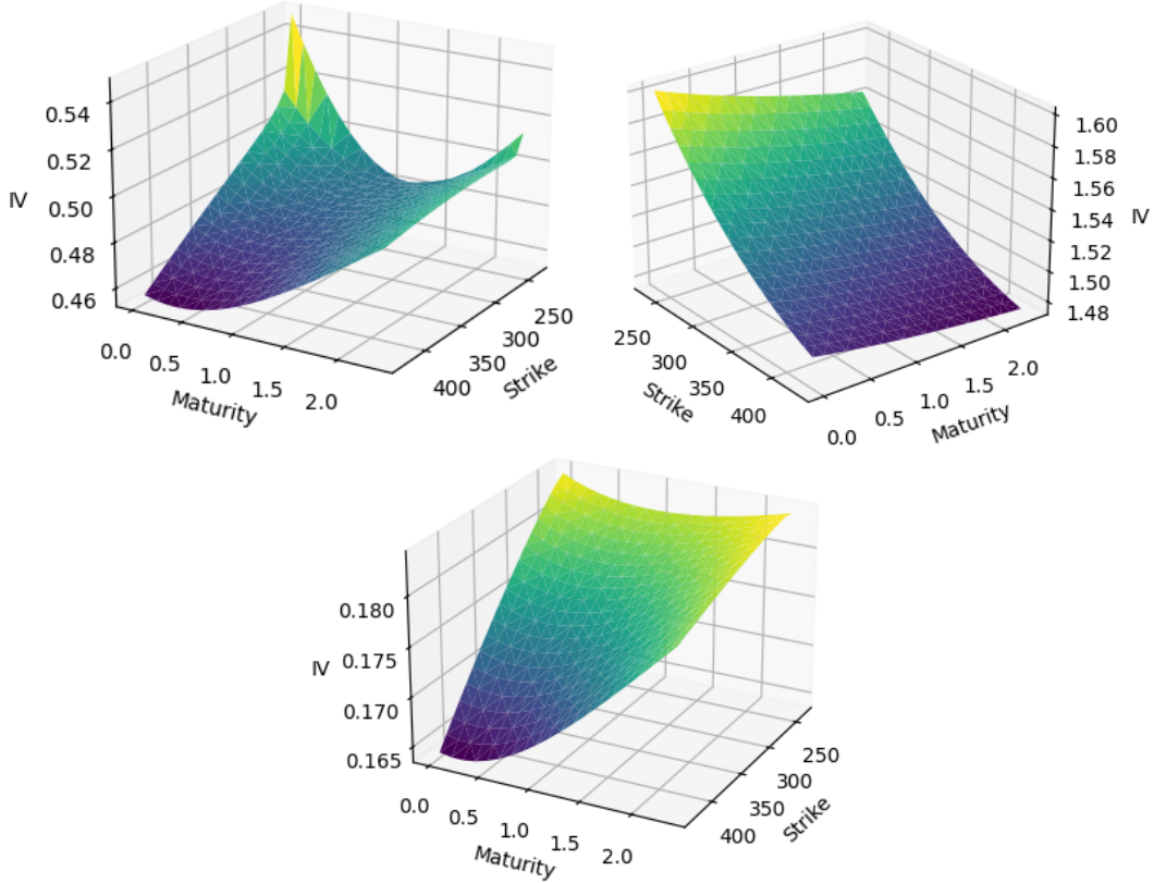
Figure 5: Surfaces for the same out-of-sample test days interpolated using the implicit scoring model for candidate selection.
