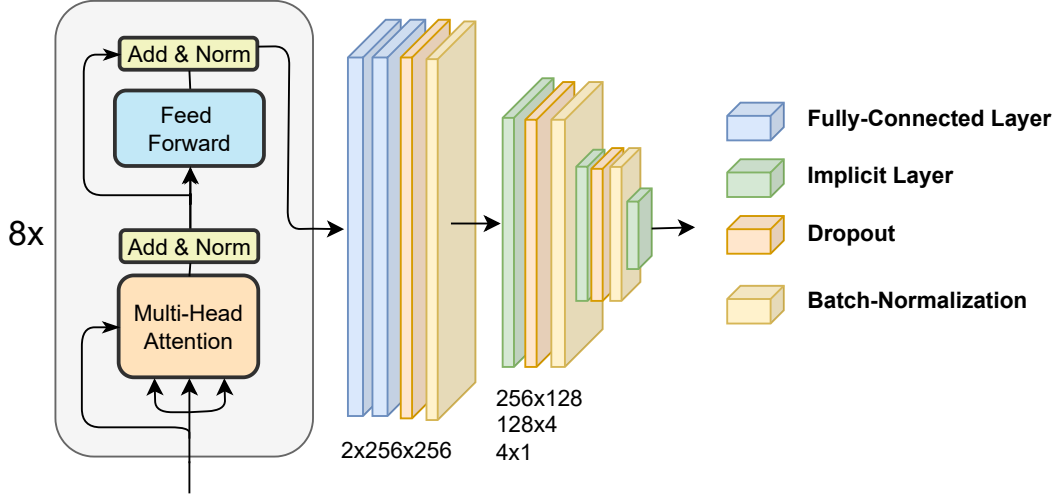
Figure 1: Visualization of the Transformer Encoder and Implicit Fixed Point Iteration Layers
