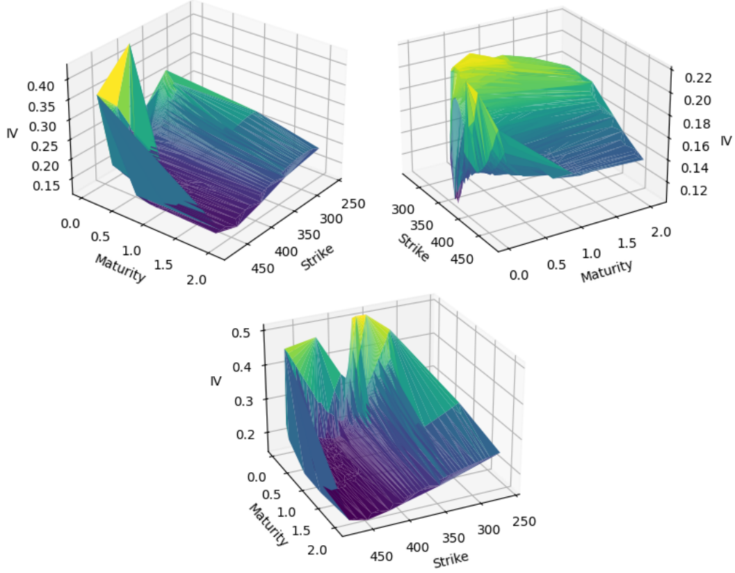
Figure 4: Surfaces interpolated on test data using a linear interpolation model.
