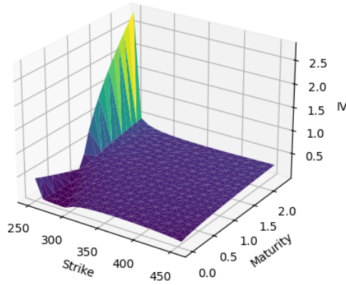
Figure 3: Surface generated using a manually optimized SABR model. Notice how the non-removal of possible outlier candidates generates a out-of-range peak in the surface.
