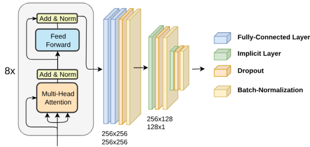
Fig. 2: Visualization of the Transformer Encoder and Implicit Layers used in the proposed architecture.
