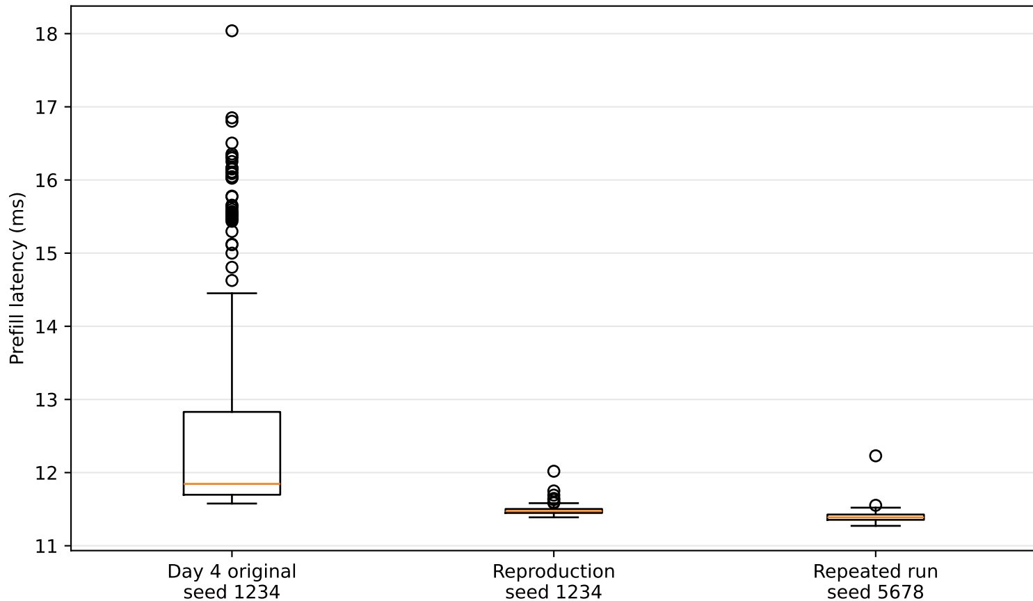
Prefill latency distribution
