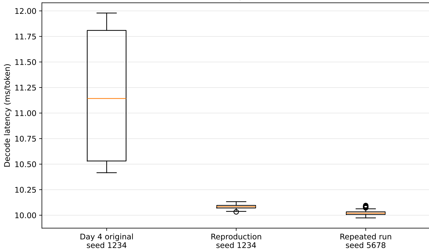
Decode latency distribution
