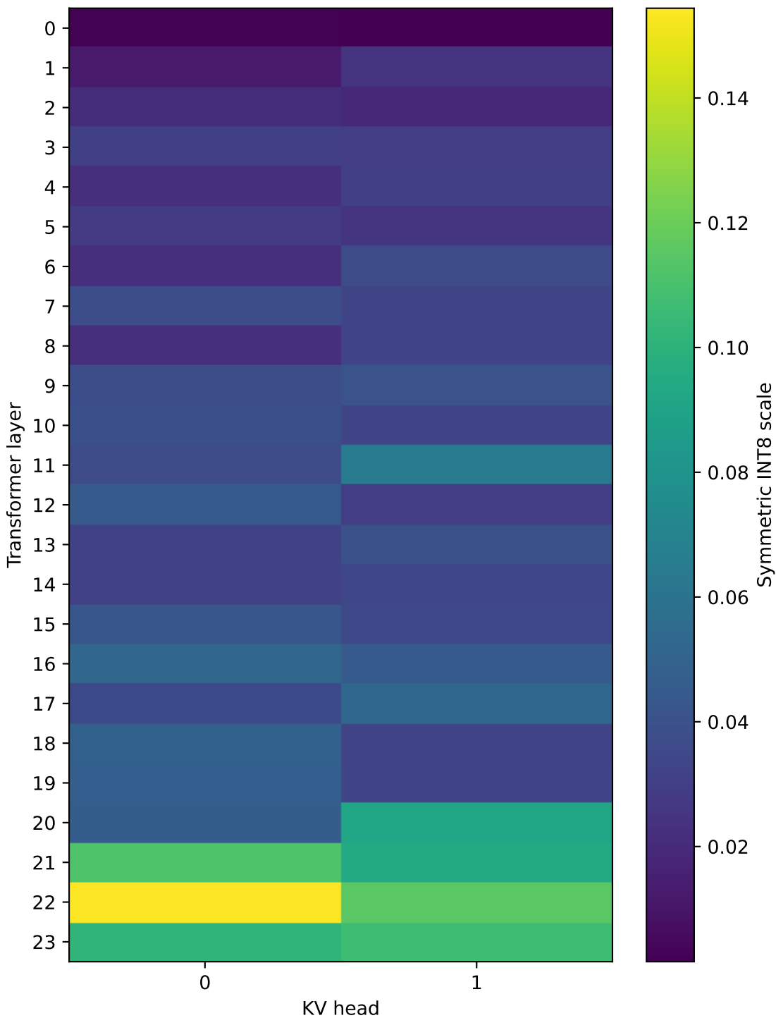
Qwen2.5-0.5B V calibration scales
