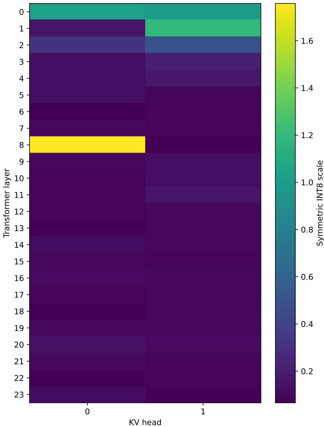
Qwen2.5-0.5B K calibration scales
