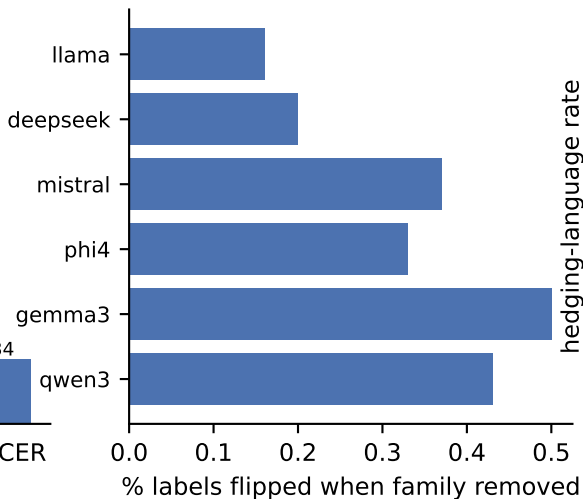
leave-one-family-out
