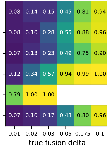
arm correlation rho = 0.8
