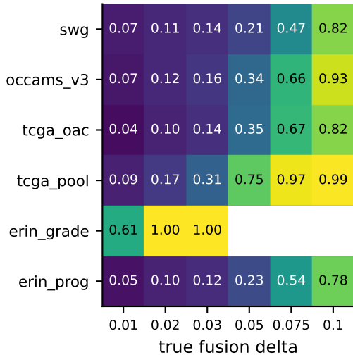
arm correlation rho = 0.6
