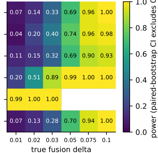
arm correlation rho = 0.9
