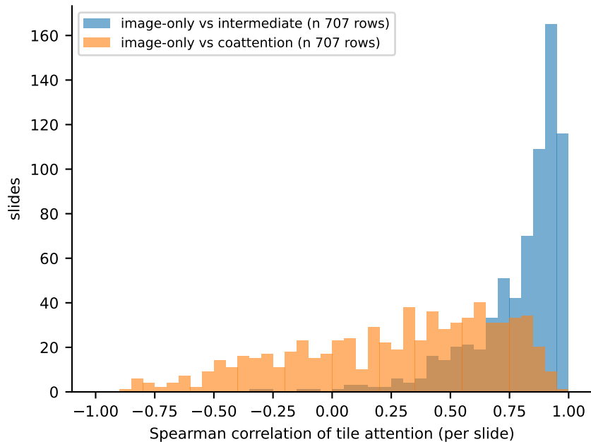
A. Attention agreement
