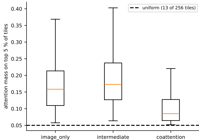
B. Attention concentration (707 slides)
