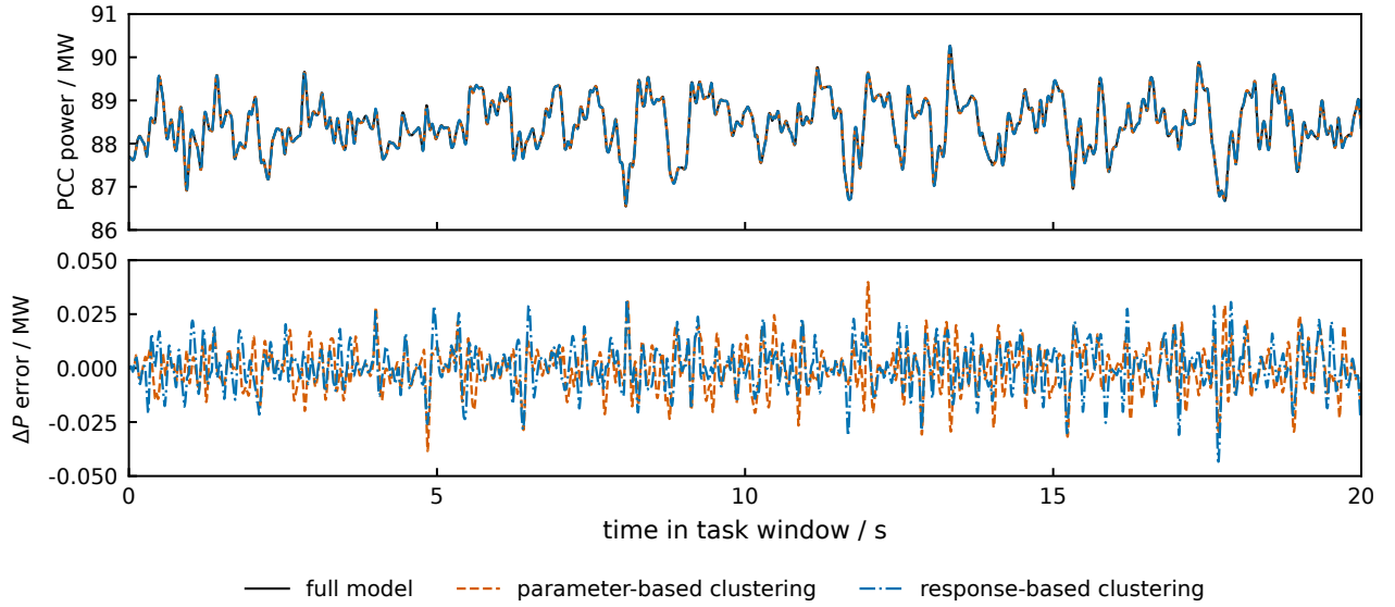
Figure S2: S2 with eight clusters under the clustering input. Both feature sets give similar PCC active-power trajectories and dynamic errors.
