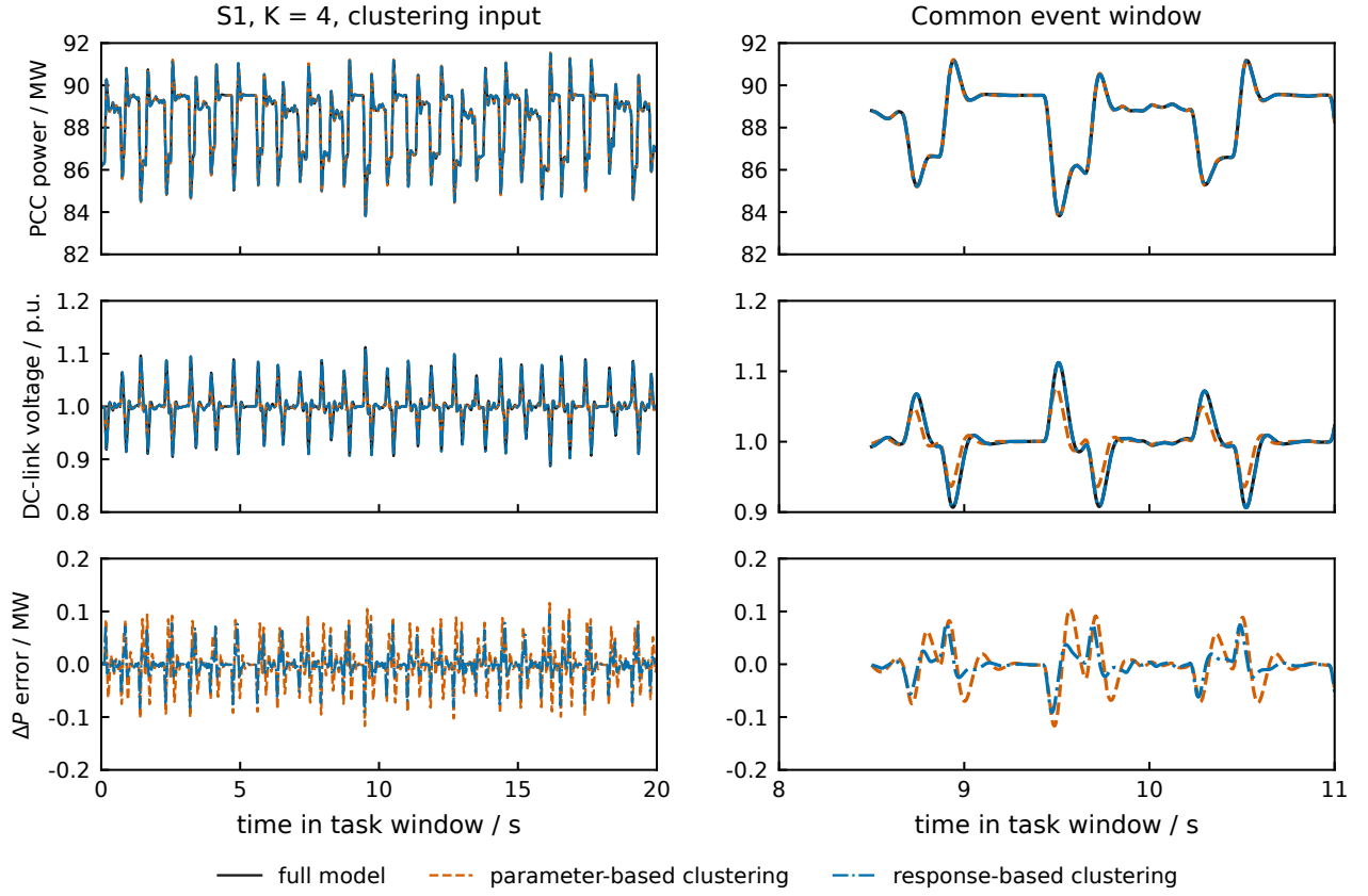
Figure S1: S1 with four clusters under the clustering input. A close PCC trajectory coexists with an inaccurate internal DC-link response. Both columns use the same models, with an overview and a common event window. The equivalent voltage is that of the chain containing the selected full-model hall.
