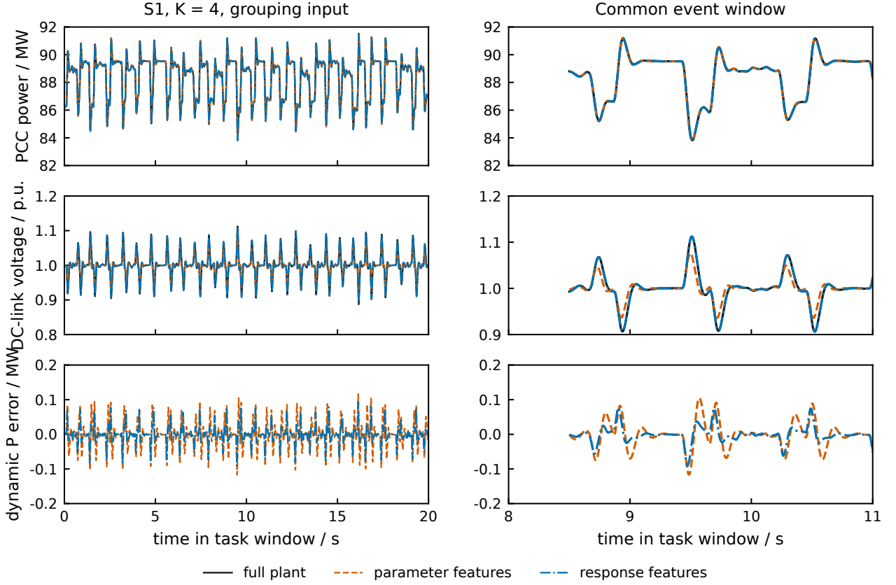
Figure S1: S1 with four groups at the grouping input. A close PCC trajectory coexists with an inaccurate internal DC-link response. Both columns use the same models, with an overview and a common event window. The equivalent voltage is that of the chain containing the selected full-model hall.
