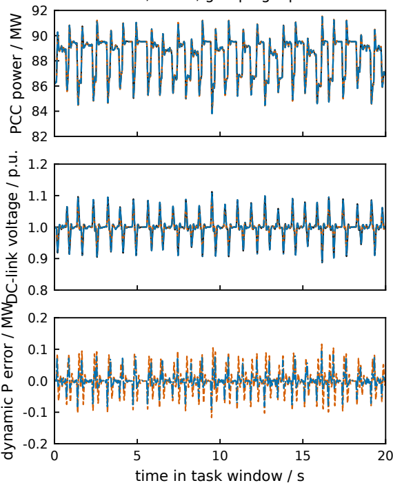
S1, K = 4, grouping input
