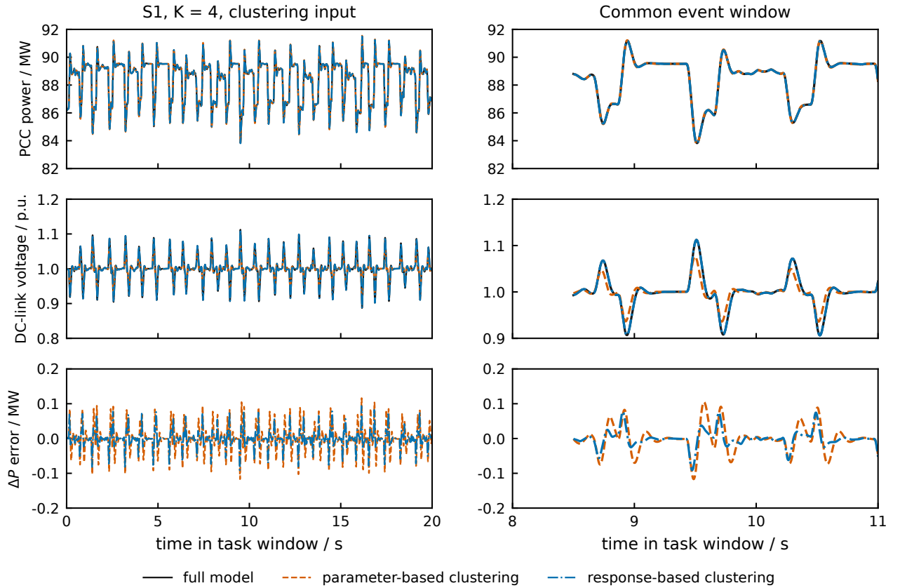
Figure S1: S1 with four clusters under the clustering input. A close PCC trajectory coexists with an inaccurate internal DC-link response. Both columns use the same models, with an overview and a common event window. The equivalent voltage is that of the chain containing the selected full-model hall.
